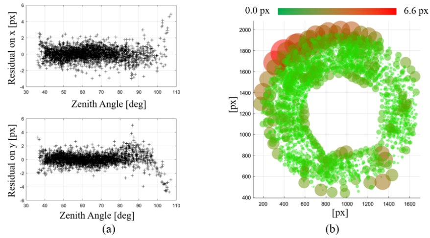
Fig. 6. (a) Distribution of the residual error on the x-axis (top) and the y-axis (bottom) (in respect of the chief ray zenith angle) applying the Scaramuzza model (b) Errors of reprojections associated to each corner for all the images of the test on the sensor plane.
