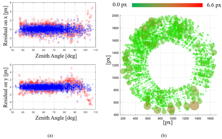
Fig. 9. (a) Distribution of the residual error on the x-axis (top) and the y-axis (bottom) (in respect of the chief ray zenith angle) applying the AME model (blue) compared to Scaramuzza one (red) (b) Errors of reprojections associated to each corner for all the images of the test on the sensor plane.
