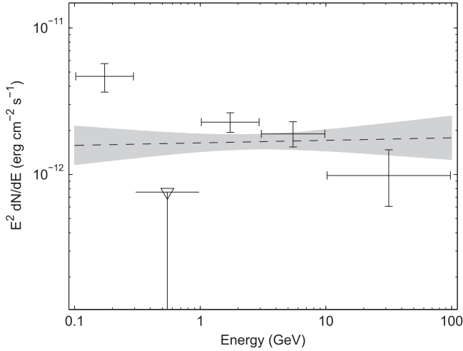
Figure 9. Spectral energy distribution of 3FGL J1226.9-1329 (PMN J1226-1328) flagged with bad spectral fit quality (Flag 10 in Table 3). The first two points deviate from the power-law fit. This source is within 1:3 of the much brighter pulsar PSR J1231-1411, so it is confused with it (within r_{68} ) below 600 MeV.
