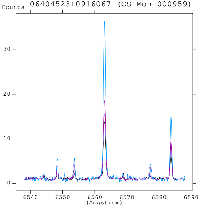
Fig. 7. Variability of the spectrum near the H\alpha emission line of the OH\alpha NA not-flagged class II accretor 06404523+0916067 for the original spectra with FWZI greater than pure nebular contribution: different colours correspond to spectra collected in different observations of the same object.
