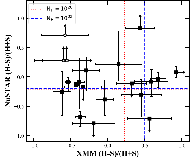
Figure 15. NuSTAR hardness ratio (with 1\sigma errors) as a function of their XMM-Newton counterpart hardness ratio (with 1\sigma errors). Expected hardness ratio values of spectral models of N_H = 10^{20} \text{ cm}^{-2} (red dotted line) and 10^{22} \text{ cm}^{-2} (blue dashed line) at z = 0.734 of NuSTAR and XMM-Newton are plotted. ID 31 has two XMM-Newton counterparts, and they are plotted in open squares. ID 33 is plotted in open circle.
