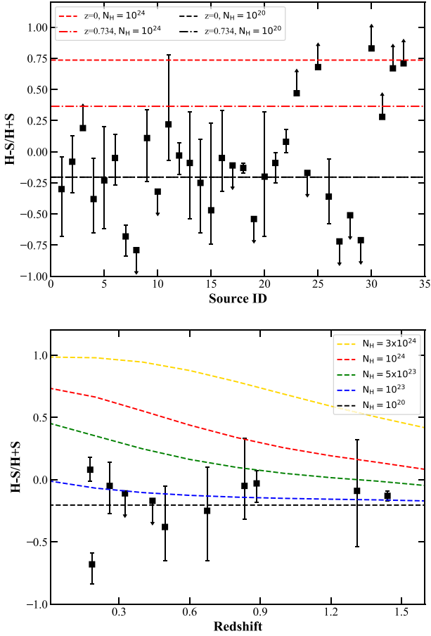
Figure 14. Upper: Hardness ratios (with 1\sigma errors) of the 33 sources in the 95 percent reliability catalogue. Expected values of spectral models of N_H = 10^{24} \text{ cm}^{-2} (red) and 10^{20} \text{ cm}^{-2} (black) at z = 0 (dashed line) and z = 0.734 (dash-dot line) are plotted. The expected values of 10^{20} \text{ cm}^{-2} at two redshifts are similar, so that the two lines overlap. Lower: Hardness ratio (with 1\sigma errors) as a function of redshift. Dashed lines show the expectations using absorbed power law models with \Gamma = 1.80 and different intrinsic column densities of 3 \times 10^{24} , 10^{24} , 5 \times 10^{23} , 10^{23} , and 10^{20} \text{ cm}^{-2} (from top to bottom) as a function of redshift.
