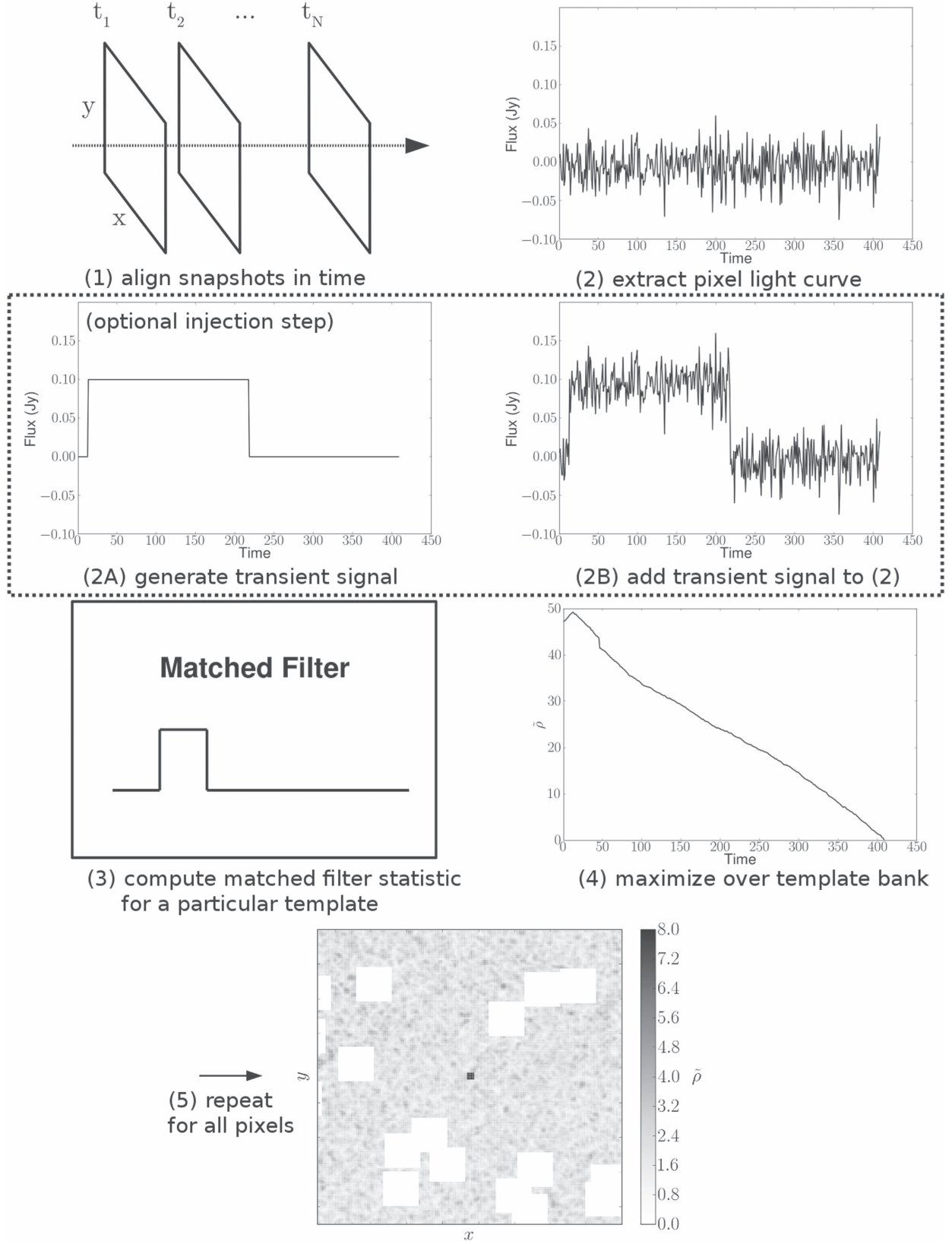
Figure 14. Illustration of the Simetra pipeline. The color scale of \tilde{\rho} has been cut off at 8. The white boxes are the locations of masked bright sources. See text for details.
