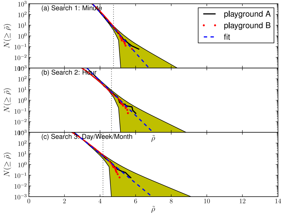
Figure 7. Cumulative background distribution of \tilde{\rho} for the playground region for the three searches. The blue dashed line is an exponential fit to the tail of the playground A distribution, where the tail consists of 100 points to the right of the vertical dotted line. The yellow shaded region is the \sqrt{N} error region for the fit, showing that the distributions from playground A and playground B agree within the error bars. All curves are normalized to the number of synthesized beams in playground B. The fit determines \tilde{\rho}^* at a predetermined P_{FA} = N(\geq \tilde{\rho}) for N(\geq \tilde{\rho}) \ll 1 when it is normalized to the number of synthesized beams in the search region. See text for further discussion.
