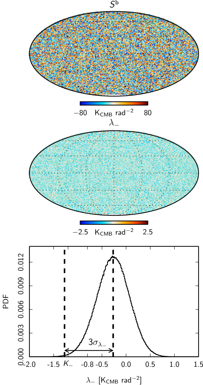
Fig. A.1. Filtered realization of the Gaussian dust sky (upper panel) and the corresponding eigenvalue \lambda_- (middle panel). The distribution of the eigenvalue \lambda_- over the unmasked pixels is Gaussian.
