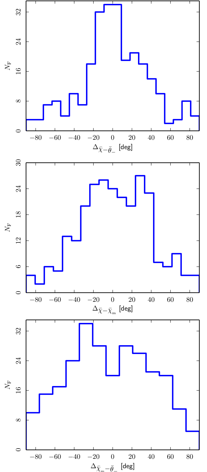
Fig. 6. Upper panel: HRO between the filaments and \mathbf{B}_{\text{POS}} . Middle panel: HRO between \mathbf{B}_{\text{POS}} and \mathbf{B}_{\text{m,POS}} . Lower panel: HRO between the filaments and \mathbf{B}_{\text{m,POS}} .
