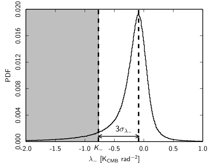
Fig. 3. Distribution of the eigenvalues \lambda_- over the unmasked pixels in the high-latitude sky. The grey region represents the pixels that were used in the SMAFF algorithm to find strong filaments.
