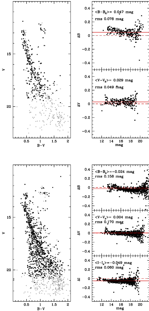
Figure 3. Comparison between our photometric catalogue and the literature ones. Upper panels: on the left the V, B-V CMD from Kaluzny & Mazur (1991) in black and our CMD on a area of the same size in gray; on the right the comparison of B and V magnitudes. The average differences and rms are indicated in the respective panels. Lower panel: the same, but with the BVI photometry from Ann et al. (1999).
