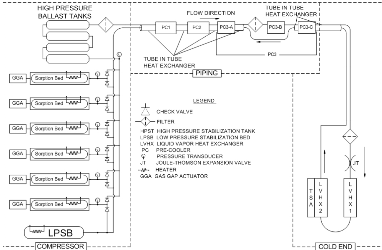
Figure 3-1 TMU schematic
