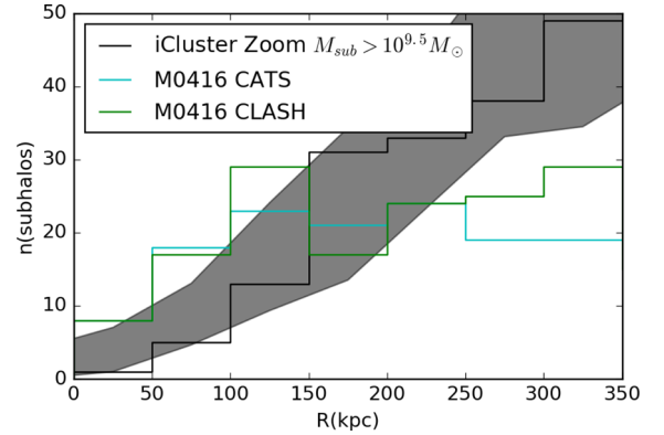
Figure 18. Comparison of subhalo properties in MACSJ 0416 inferred from lens modelling in this work and from the CLASH collaboration (Grillo et al. 2015) with that derived from the 10^{15} M_\odot cluster from the Illustris suite – the radial distribution of subhaloes.
