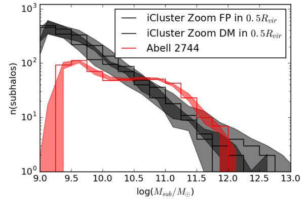
Figure 4. Comparison of the SHMF derived for Abell 2744 (with overplotted modelling errors derived from the dispersion in N -Bayesian realizations for the key fiducial parameters r_{t*} and \sigma_{0*} ) with dark matter only and full physics Illustris iCluster Zooms : the SHMF derived from the HSTFF data (red histogram) for Abell 2744 is plotted along with that derived from the iCluster Zooms . The DM-only run is plotted as a solid black histogram with the dispersion marked in the dark grey band and the full physics run (grey histogram) and corresponding dispersion shown as the light grey band. Subhaloes within 0.5 R_{\text{vir}} that corresponds to the FOV of ACS over which the lensing model has been reconstructed are extracted from iCluster Zoom 1 . The full physics run of iCluster Zoom 1 includes subgrid models for the physical processes that are relevant to galaxy formation. From the full physics run, we have selected only subhaloes that host a stellar component.
