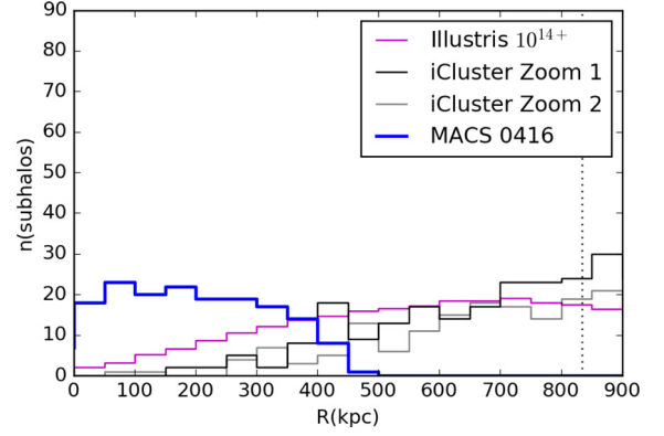
Figure 17. Radial distribution of the SHMF derived from simulated Illustris clusters ( 10^{14} Illustris Haloes ) as well as the two zoomed-in runs iCluster Zooms compared to that of the lensing-derived SHMF for MACSJ 0416 from the HSTFF data (blue histogram). Once again the most massive 117 simulated clusters selected at z = 0.3-0.5 from the 10^{14} Illustris Haloes and the two massive zoomed-in cluster snapshots of the full physics run were selected. As clearly seen from the radial distribution of the count-matched subhaloes that galaxies in Illustris are not as centrally concentrated as MACSJ 0416. The radial distribution of subhaloes in Illustris are significantly more diffuse even when compared to the iCluster Zooms .
