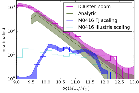
Figure 14. Comparison with the analytically predicted SHMF: the lensing derived SHMF (with model errors) for the two independent scaling laws is overplotted along with the analytically calculated SHMF for a cluster halo with mass equivalent to that of MACSJ 0416. This analytic estimate includes the halo-to-halo scatter that is shown in the dull green band.
