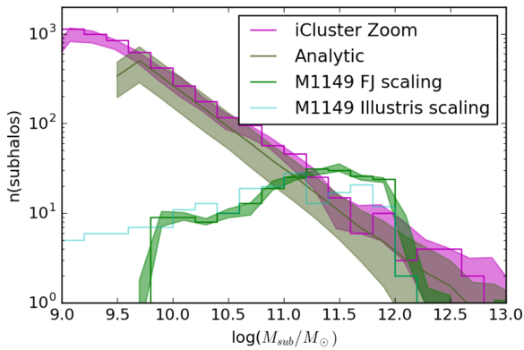
Figure 23. Comparison with the analytically predicted SHMF: the lensing-derived SHMF (with model errors) for the two independent scaling laws is overplotted along with the analytically calculated SHMF for a cluster halo with mass equivalent to that of MACSJ 1149. This analytic estimate includes the halo-to-halo scatter that is shown in the dull green band. Note that the excess in substructure abundance seen in the mass range between 10^{11} and 10^{12} M_{\odot} cannot be fully accounted for with cosmic variance alone.
