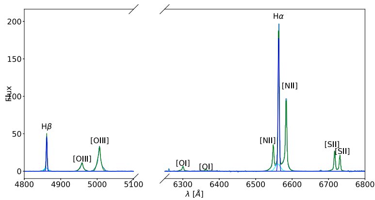
Figure D12. IRAS 21453–3511.
