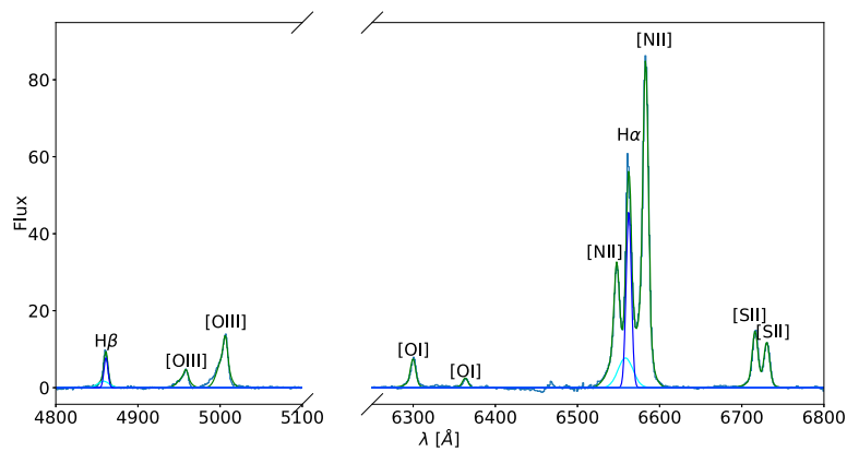
Figure D9. IRAS 19542+1110.
