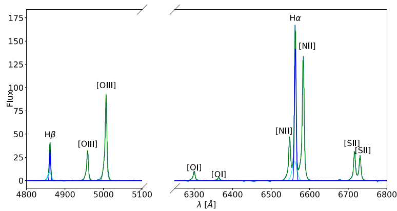
Figure D7. IRAS 13229–2934.
