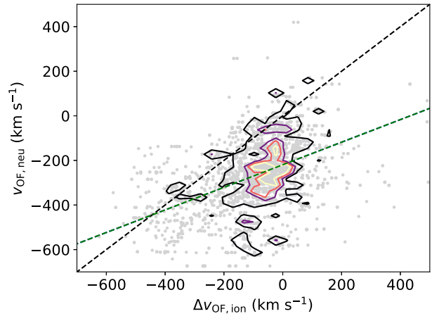
Figure 9. Neutral outflow velocity ( v_{50} ) versus ionized outflow blueshift for all spaxels of all galaxies. The coloured isodensity contours correspond to 10, 30, 50, and 70 points in that bin (the parameter space has been divided into 50 bins). The dashed black line indicates the 1:1 correlation, the green dashed line is the best fit to the data points.
