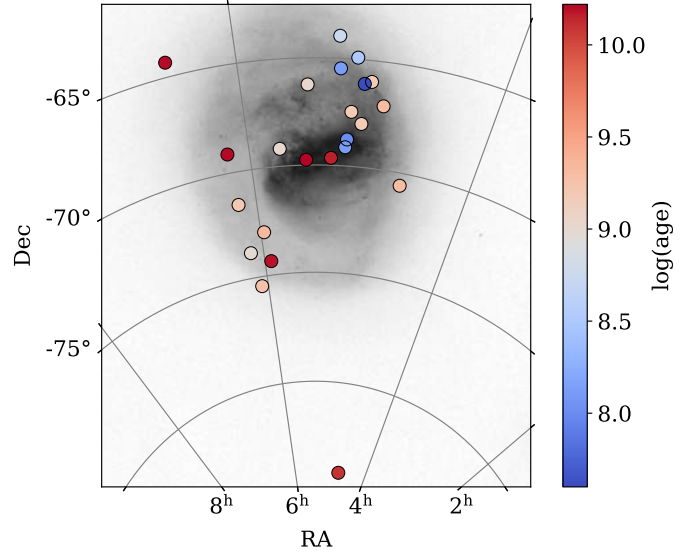
Fig. 1. Spatial distribution of the 23 LMC star clusters in our sample, colour-coded by their age. The background grey-scale image shows a stellar density map from Gaia DR3.
