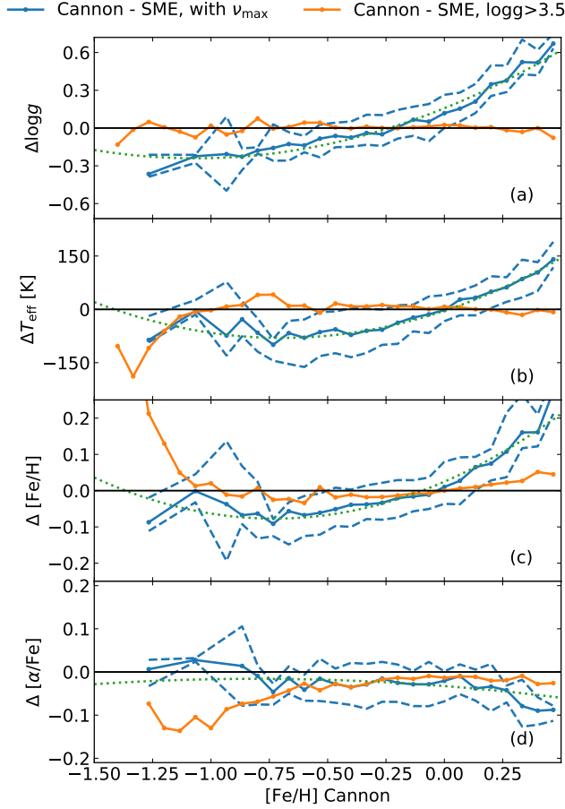
Figure 9. Comparison of GALAH-DR2 Cannon-based (data-driven) estimates to that of SME-based (model-driven) estimates. The plots show systematic trends as a function of Cannon-based iron abundance [\text{Fe}/\text{H}] . The giants (blue) and dwarfs (orange) are shown separately. The giants shown are seismic giants from K2, and for them SME was run using \nu_{\text{max}} estimated from asteroseismology as a prior. The seismic giants show strong systematic trends while dwarfs have negligible systematics. The dotted line is a two degree polynomial fit to the trends for the seismic giants with -1.5 < [\text{Fe}/\text{H}] < 0.3 .
