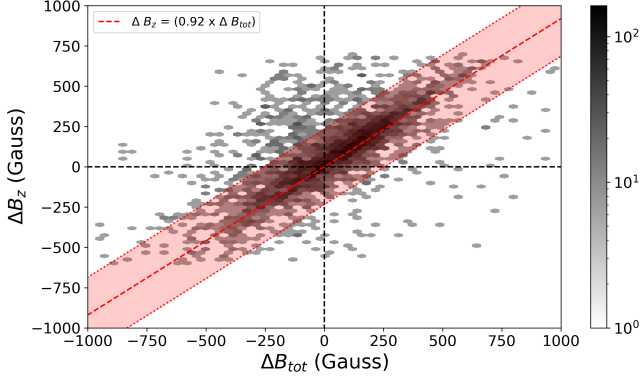
Figure 6. The fluctuations in B_z (i.e., \Delta B_z ) arising from the development of a shock, plotted as a function of the change in the total magnetic field strength ( \Delta B_{\text{tot}} ) also produced from the commencement of the shock. The shade of each hexagon represents the density of points within that region. The vertical and horizontal dashed black lines highlight magnetic field fluctuations equal to 0 Gauss. The dotted red line displays the linear line of best fit, with the shaded red region (bounded by small dotted red lines) indicating the 1\sigma errors associated with the fit.
