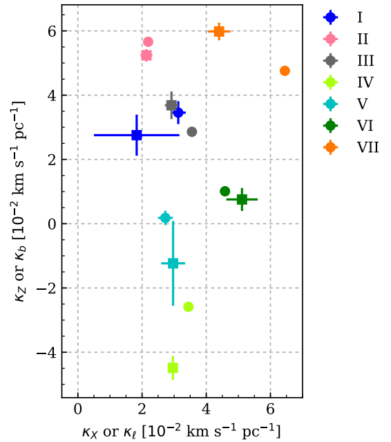
Fig. 5. Observed linear expansion rates (as listed in Table 1). Squares: ( \kappa_X, \kappa_Z ) from 3D velocities. Dots: ( \kappa_\ell, \kappa_b ) from corrected tangential velocities (see Sect. 3.2). The colour-coding is the same as in Figs. 3 and 4.
