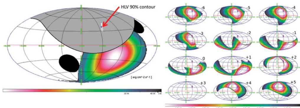
Figure 4. The GRID 2\sigma UL map (in 30 MeV – 10 GeV) on 4 s integration around GW170814 T_0 , showing the LR occulted by the Earth (left panel). The 150 s exposure UL map scan preceding and following T_0 (right panel) evaluated at the optical transient position.
