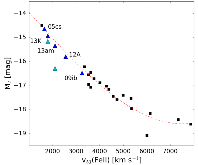
Figure 5. Velocity–luminosity relation for a sample of nearby Type II SNe collected by Nugent et al. 2006 (black squares; their table 4). The fit to the data (dashed red line) is their equation (1). The blue triangles are SNe 2005cs, 2009ib, and 2012A (Pastorello et al. 2009; Tomasella et al. 2013; Takáts et al. 2015), and SNe 2013K and 2013am (this work). For the latter two SNe, the cyan triangles are before applying the extinction correction.
