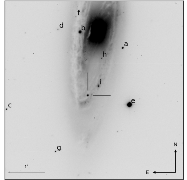
Figure 2. SN 2013am and local sequence stars (Liverpool Telescope, g -band image obtained on 2013 March 30, with exposure time 180 s).
