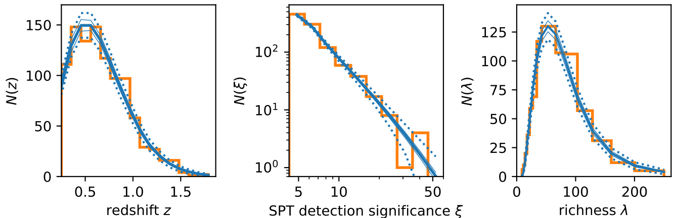
FIG. 1. Projection of the 1,005 clusters in the SPT sample along the dimensions of redshift, SPT detection significance, and optical richness. Orange histograms show the data. Thick lines show the mean recovered model in an analysis of the cluster abundance and cluster lensing, thin solid lines show the 1\sigma uncertainty on the mean, and dotted lines show the 1\sigma Poisson uncertainty (statistical shot noise). There is qualitative agreement between the model and the data.
