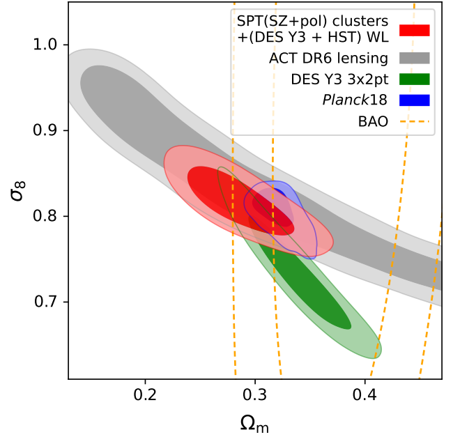
FIG. 7. Constraints on \Omega_m and \sigma_8 (68% and 95% credible regions) in a \Lambda CDM universe with massive neutrinos from the abundance of SPT clusters, a selection of large-scale structure lensing probes [9, 17], Planck primary CMB measurements (TT,TE,EE+lowE) [2], and BAO [96–99]. Our measurement of the cluster abundance places competitive constraints especially on S_8^{\text{opt}} .
