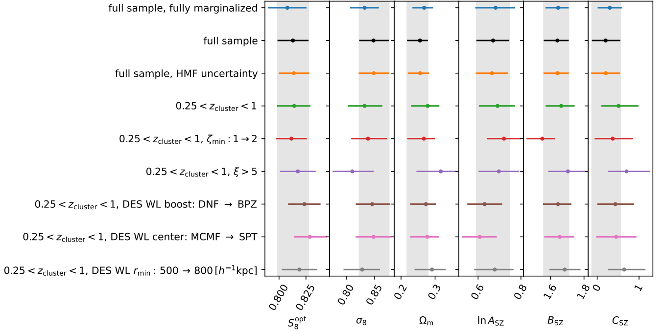
FIG. 3. Impact of different analysis choices on the constraints on key cosmological and SZ–mass relation parameters (mean and 68% credible interval), assuming a \Lambda CDM model. During the blinded phase of the analysis, the parameter values were artificially offset by an unknown amount. The vertical gray bands show the 68% credible interval of the “full sample” analysis (second row) for reference. All results shown here are based on mass calibration using only the DES Y3 lensing data, the HST-39 lensing data are not used. Only the results in the first row shows constraints that are marginalized over all nuisance parameters; for simplicity, for all other tests, we fix the parameters of the M_{\text{WL}}-M_{\text{halo}} relations, the intrinsic scatter correlation coefficients, and \Omega_\nu h^2 , \Omega_b h^2 , and n_s to their nominal values. DNF and BPZ are two redshift estimators that we use to determine the amount of cluster member contamination in the lensing signal. MCMF and SPT refer to cluster centers as measured in optical data by MCMF or as determined in the SZ analysis of SPT data.
