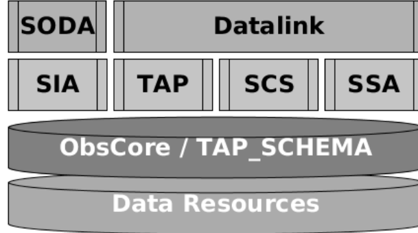
Figure 4. Simplified view of a subset of Data Access Layer services on top of a (generic) data resource. Three layers on top of the data resource are sketched: a metadata content layer (ObsCore/TAP_SCHEMA), a dataset discovery one (SIA, TAP, SCS and SSA, even if SCS, the Simple Cone Search actually performs data access directly), and a dataset access (SODA and DataLink).
