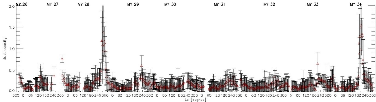
Fig.3. Zonal mean dust opacity averaged for a region from 40.5°S to 40.5°N as a function of L_s . The data are binned in L_s of 3^\circ . Dust opacity is normalized to the reference pressure 6.1 mbar. Standard deviations contain variabilities of dust opacity within each bin. An “error bar” represents the standard deviation of each averaged value and provide an indication of the observed zonal and meridional variations.
