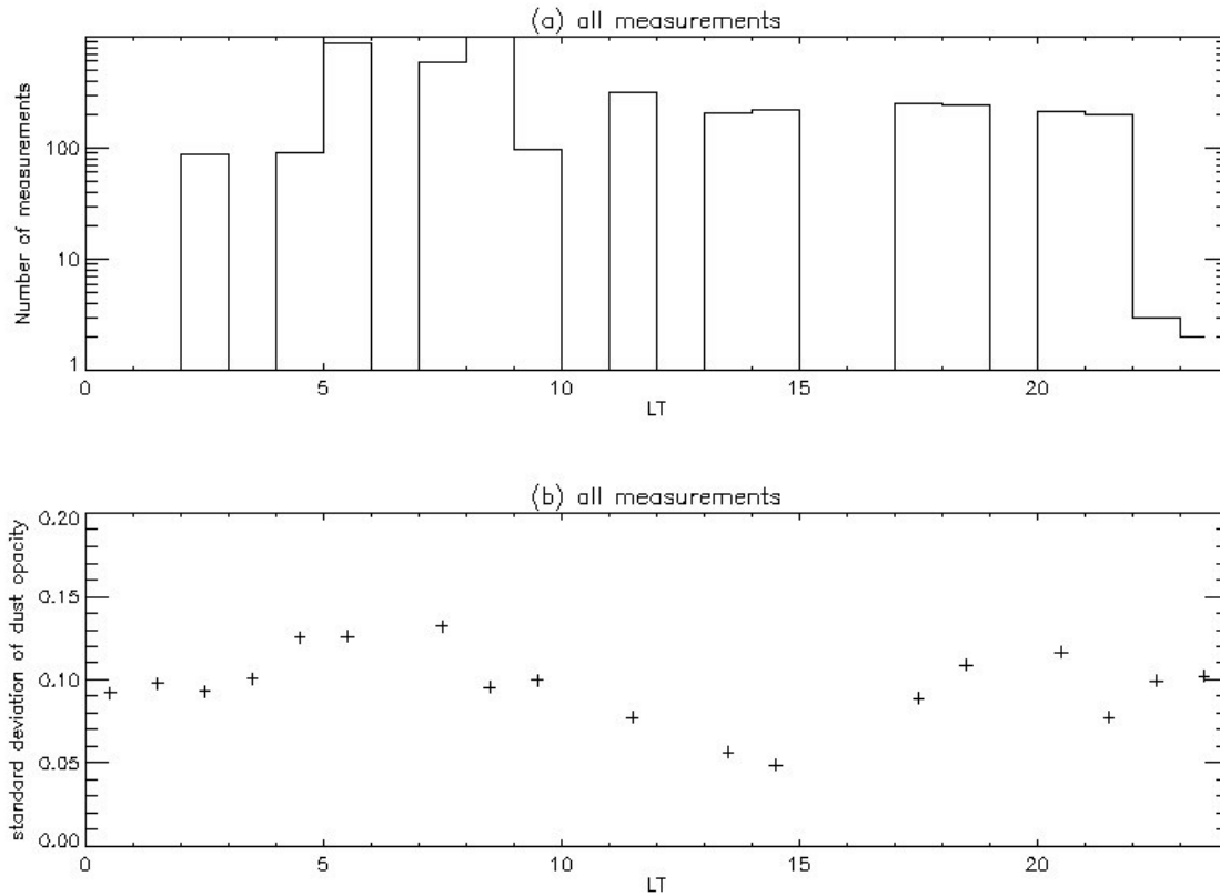
134 135 Fig. 1. Histogram of standard deviations for dust opacity: (a) number of measurements as a function 136 of LT, (b) standard deviations of dust opacity as a function of LT. Gaps in Fig.1b mean no 137 measurements.
