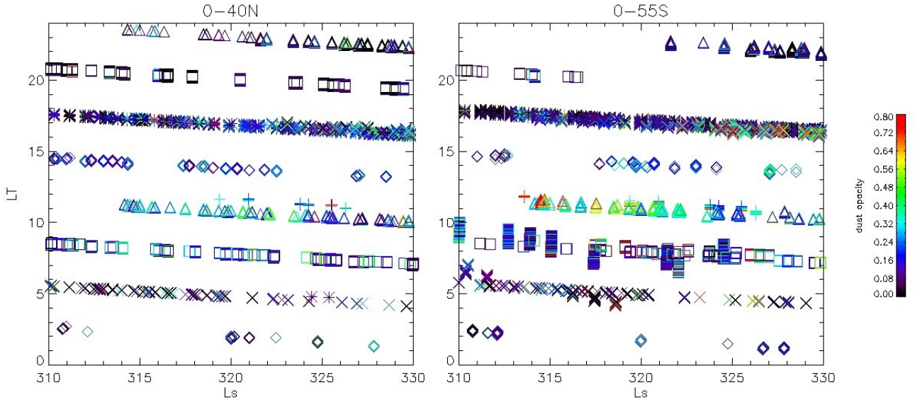
Fig.15. Dust opacity as a function of Ls and LT in different MYs for C storms a) 0 – 40°N and b) 0 – 55°S. Different symbols correspond with different MYs as in the legend of Fig. 12.
