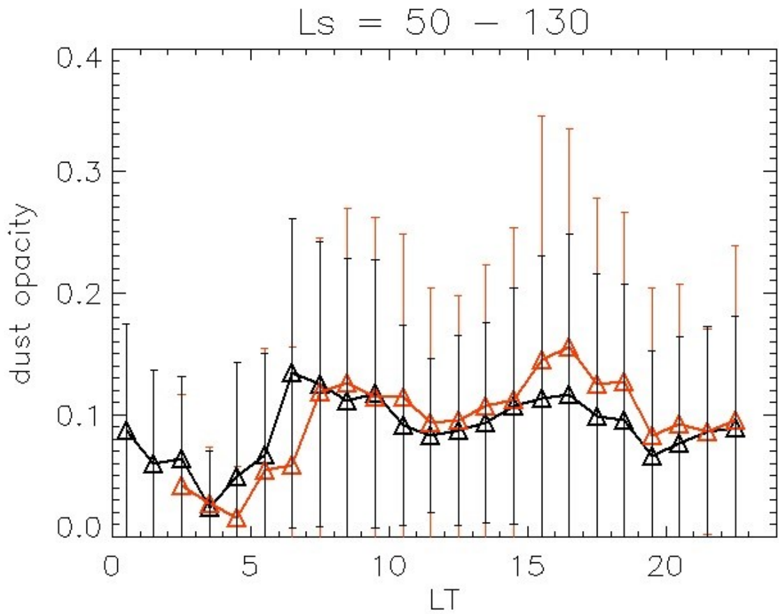
Fig.16. The dust variation with LT for Ls interval from 50° to 130° on either side of the northern summer solstice. Data binned with 1-hour bin and collected for the southern (0 - 25°S) and northern hemispheres (0 - 25°N) are plotted by red and black triangles, respectively. The “error bars” represent the standard deviation of each averaged value and provide an indication of the observed zonal, meridional, and inter-annual variations.
