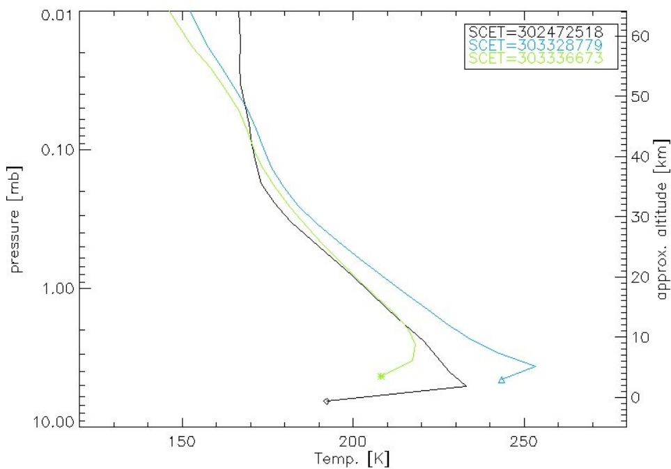
Fig.B2. Temperature profiles extracted from EMCD v5.3 for atmospheric conditions similar to three PFS measurements in MY31. Black line corresponds to the PFS measurement (SCET 302472518) taken at 18.81 LT, Ls = 217.38, latitude 16.77N and longitude 15.52E. Blue line corresponds to the PFS measurement (SCET 303328779) taken at 18.32 LT, Ls = 223.52, latitude 28.18S and longitude 136.69E. Green line corresponds to the PFS measurement (SCET 303336673) taken at 6.18 LT, Ls = 223.58, latitude 28.6S and longitude -73.14E. Symbols mean surface temperatures for each measurement.
