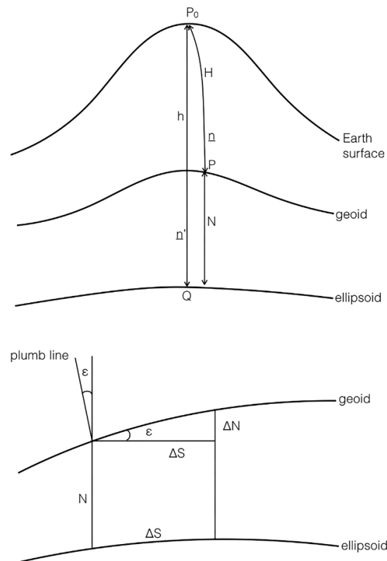
Figure 3. Relation between the geoid undulation N and the deflection of the vertical \varepsilon . (Adapted from [27]).
