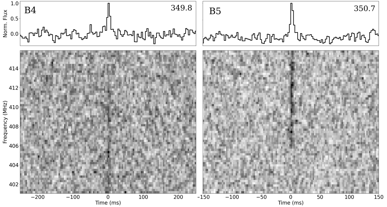
Fig. 2. Bursts from FRB 20180916B observed on April 30th 2022 (left panel) and August 9th 2022 (right panel), respectively. Bottom panels show the dynamic spectra, while the top panels show the frequency averaged profiles. The best-fit DMs (in \text{pc cm}^{-3} ) at which the bursts were de-dispersed are reported in the top right corner of each plot. Data were down-sampled to have 64 frequency channels, each 0.25 MHz wide, and time bins with 2.2 ms width for better display.
