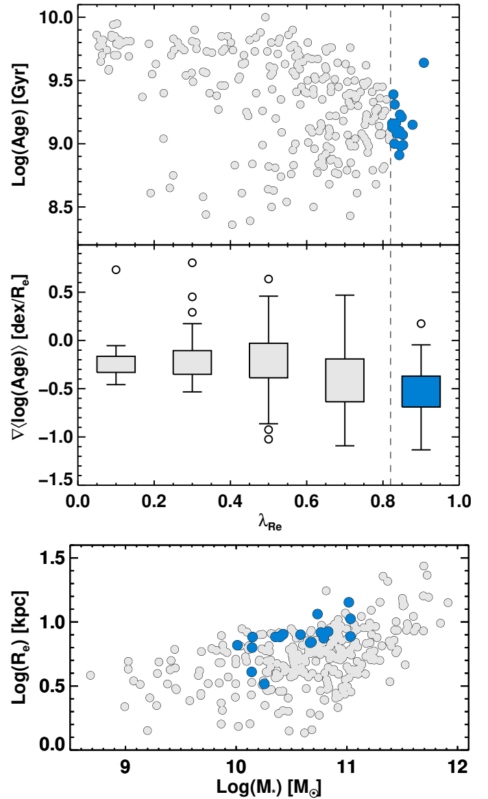
Fig. 6. Top and middle panels: \lambda_{\text{Re}} relations with mean age within R_e , mean stellar age gradient within R_e for our sample of CALIFA galaxies. Bottom panel: stellar mass–size relation. The whisker plot in the middle panel was computed in the same way as in Fig. 5. Galaxies above the 95% percentile of \lambda_{\text{Re}} distribution of the sample are marked in blue. The dashed line in the top and middle panels marks that percentile.
