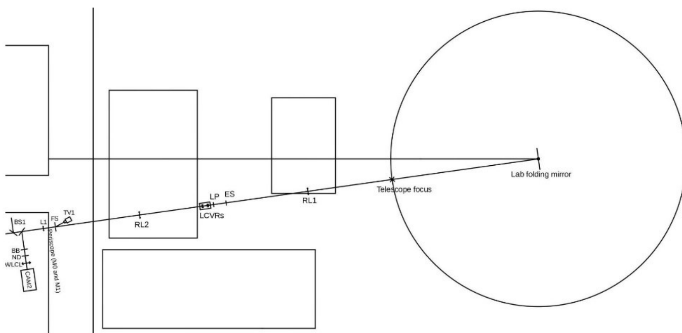
Figure 2: Optical relay system between the telescope focus and the IBIS 2.0 FS, showing the position of the two LCVRs. The rectangles are the optical tables, the circle indicates the position of the telescope focus rotatable with the Lab folding mirror.
