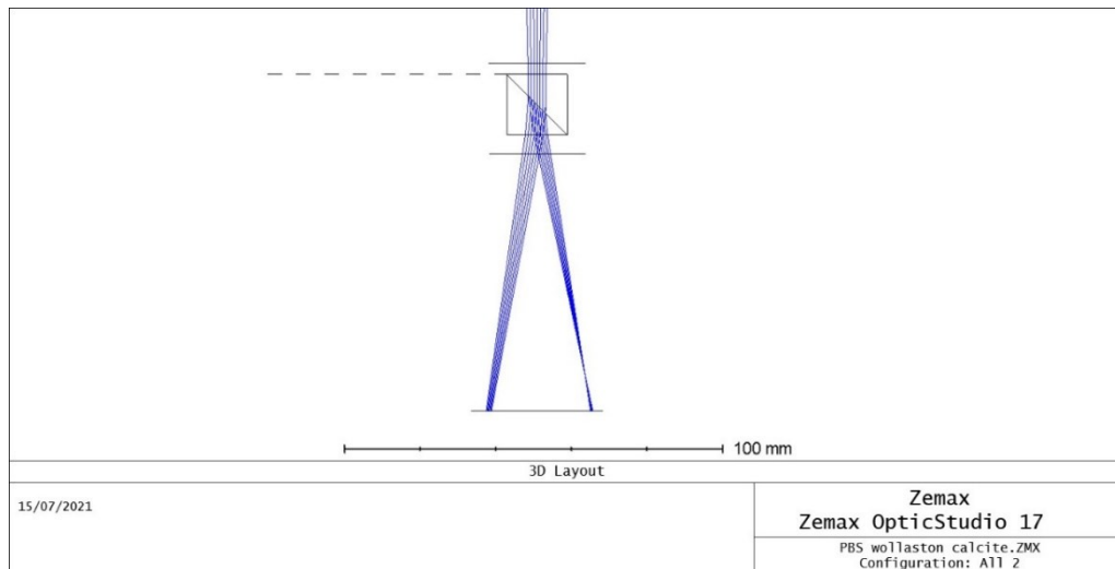
Figure 7: Wollaston prism made of calcite inserted in the convergent beam coming from L4.
