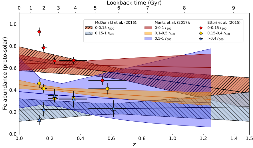
Fig. 8 Redshift evolution of the Fe abundance within different radial bins in cool-core clusters, compiled from recent works. For clarity, the scatter of the measurements are not shown. All the abundances are rescaled with respect to the proto-solar values of Lodders et al. (2009).
