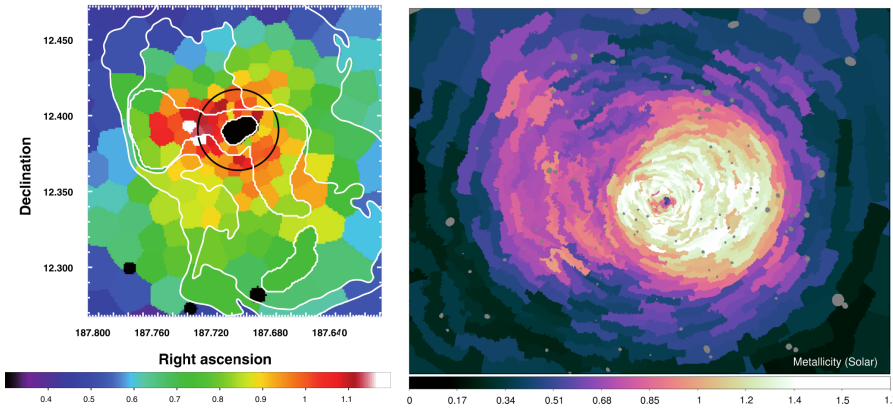
Fig. 4 Left (from Simionescu et al. 2008, reprinted with permission): Fe metal map of the giant elliptical M 87. Regions of most metal-rich gas coincide with the lobes of radio emission (white contours), suggesting an efficient uplifting by the AGN feedback. Right (from Sanders et al. 2016, reprinted with permission): Fe metal map of the Centaurus cluster, exhibiting a central abundance redistribution at larger scales via sloshing. A central drop in Fe can also be seen in the very core (see Sect. 3.1).
