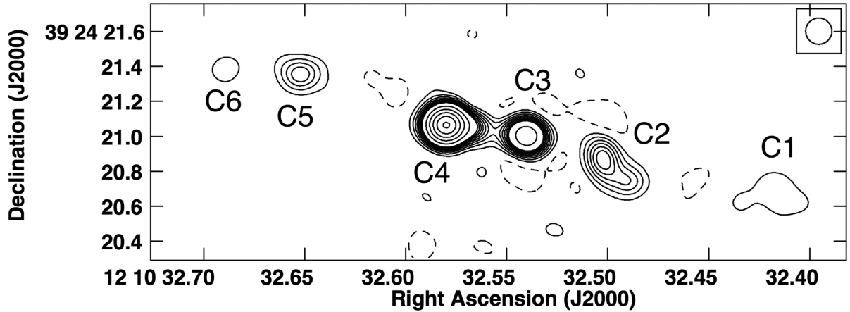
Figure 5. Same as Fig. 4 but using the new eMERLIN data and reduced with the eMERLIN cookbook. This included all seven eMERLIN antennas. As in Fig. 4, the uv -range was limited to 100\text{--}1000 \text{ k}\lambda .
