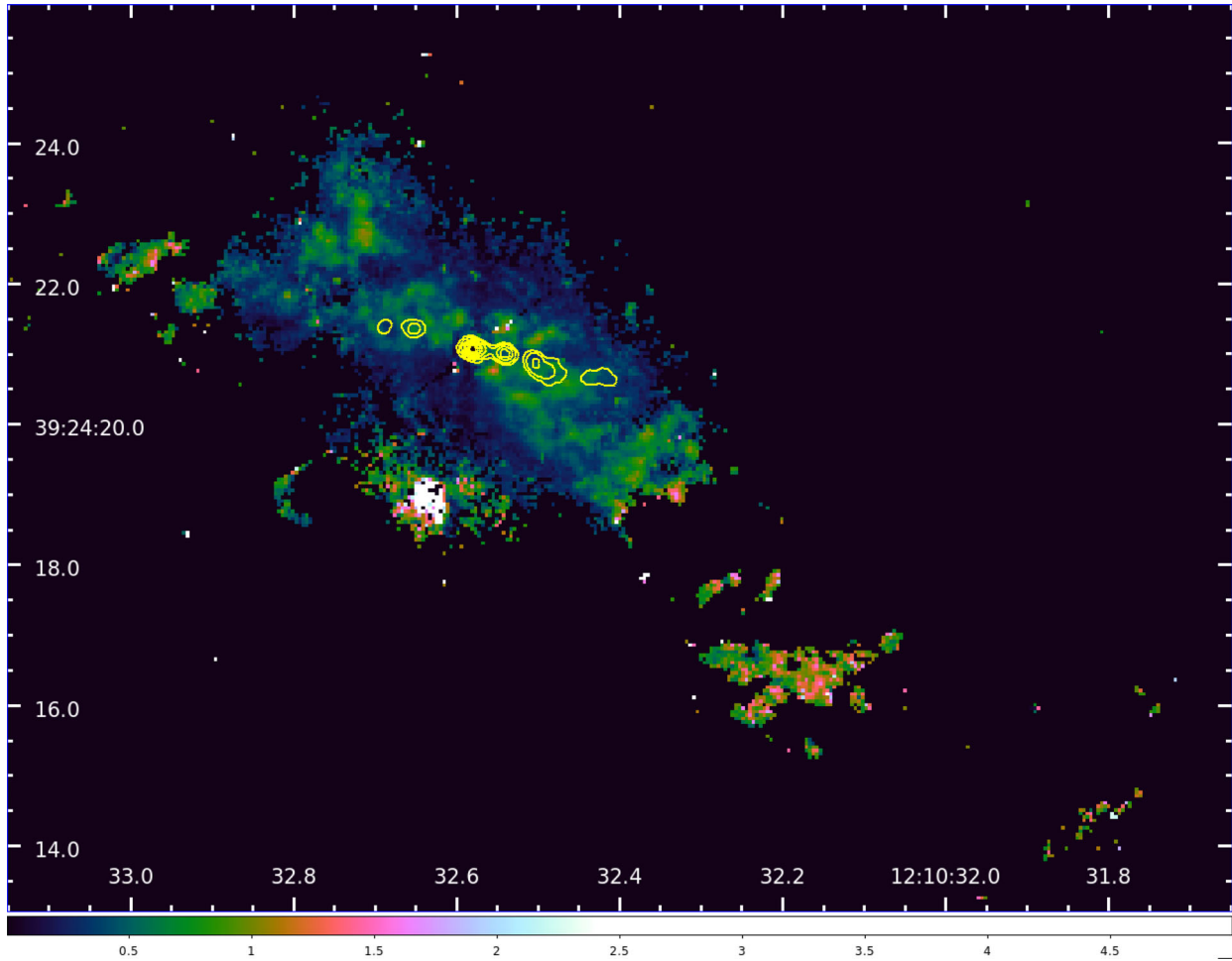
Figure 8. Image showing the ratio of the optical [O III] to H \alpha line emission from HST imaging of the central \sim 21 \times 12 arcsec 2 ( \sim 1.9 \times 1.1 kpc 2 ) of NGC 4151. The full resolution eMERLIN radio contours are plotted on top and are at 2, 4, 9, 16, 25, 36, 49 and 64 mJy beam -1 . We clipped out any pixels with S/N < 4 to remove spurious artefacts. The larger scale structure of the ionization region is seen southwest of the core. This lines up more closely with the PA of the overall line emission \sim 50^\circ but it is clear that the inner region bounded by the radio jet is at a slightly different angle at \sim 57^\circ . In this image, north is up and east is to the left.
