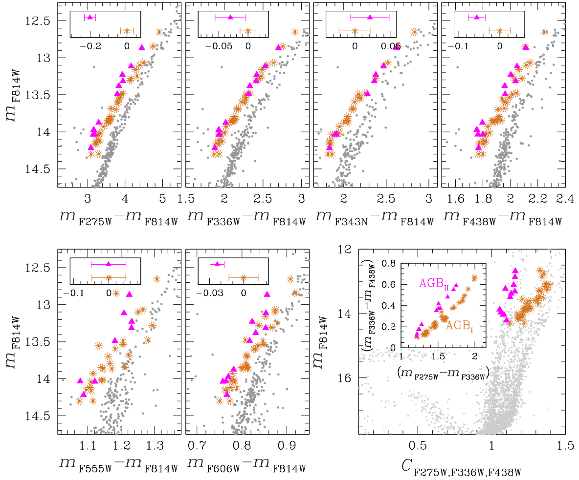
Figure 11. Analysis of AGB stars. Top-panels and first two bottom panels show the m_{F814W} versus m_X - m_{F814W} CMDs, with X = F275W, F336W, F343N, F438W, F555W , and F606W ; the inset panels show the average colour difference between AGB I and AGB II sequences. The right-hand bottom panel shows the m_{F814W} versus C_{F275W, F336W, F438W} pseudo-CMD for all the stars (grey points) and for AGB stars (coloured points). Inset panel is the m_{F336W} - m_{F438W} versus m_{F275W} - m_{F336W} two-colour diagram of AGB stars. In all the diagrams, brown starred dots and magenta triangles represent the AGB I and AGB II stars, respectively.
