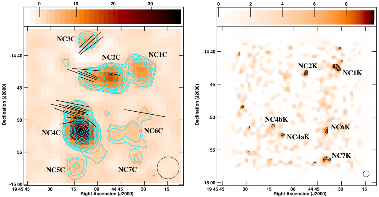
Figure 1. Left: SRT C-band total intensity 21 arcmin \times 21 arcmin image of NGC 6822 resulting from the spectral average of the inner 80 per cent of the bandwidth. The FWHM beam is 2.9 arcmin (bottom-right corner). The noise level is 0.65 \text{ mJy beam}^{-1} . Contour levels are 0.65 \times (3, 4, 6, 8, 10, 15, 20, \dots, 80) \text{ mJy} . Electric field polarization vectors are overlaid. The length of the vectors is proportional to the polarization percentage (with 10 per cent being a bar of \sim 2.1 arcmin), while their orientation represents the polarization angle. The error on the polarization angle is less than 10^\circ , and the fractional polarization is above 3\sigma_{\text{FPOL}} . Right: SRT K-band total intensity 18 arcmin \times 18 arcmin image of NGC 6822 resulting from the spectral average of the inner 80 per cent of the bandwidth. The FWHM beam is 0.9 arcmin (bottom-right corner). The noise level is 2.0 \text{ mJy beam}^{-1} . Contour levels are 2.0 \times (3, 3.5, 4, 4.5, 5, 6, 7) \text{ mJy} .
