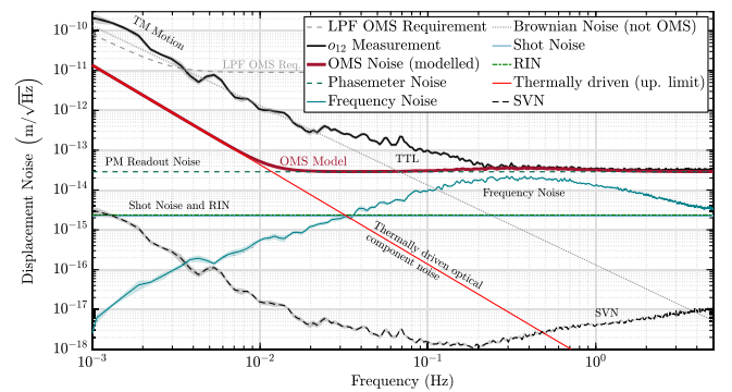
FIG. 12. Noise model applied to an o_{12} measurement from June 1st, 2016 starting at 18:46 UTC and lasting until 20:29 UTC in nominal configuration. Shown is the ASD computed with the same LPSP algorithm as in Fig. 5. Below 20 mHz TM motion caused by Brownian force noise dominates the noise spectrum. Modified from [1] by including SVN. We see that this noise contribution has negligible impact due to the implemented mitigation strategies.
