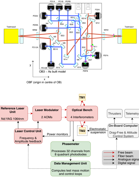
FIG. 2. Top panel: The four interferometers on the OB. The Optical Bench Frame (OBF) has its origin in the center of the OB. Bottom panel: Schematic overview of the OMS and its main components (reprint from [1] for convenience).
