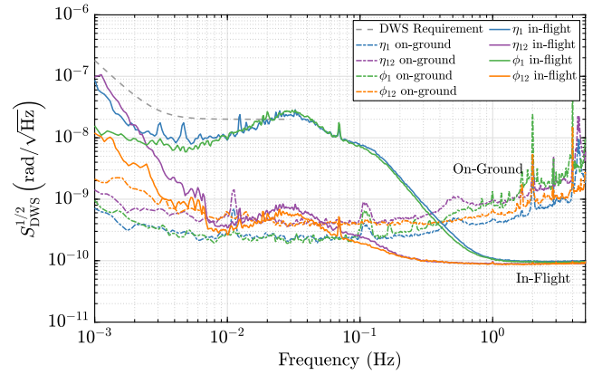
FIG. 6. Comparison of interferometric measurements on-ground and in-flight of the angular DWS TM readouts together with the noise requirement. The spectral shape is similar to the longitudinal measurements but has contributions from real TM movements (independently validated by low frequency (<mHz) capacitive sensing), SC jitter, star-tracker noise and OMS sensing noise. The latter is computed from the pseudoflat noise at high frequencies. This figure has been produced using the same LPSD algorithm as in Fig. 5.
