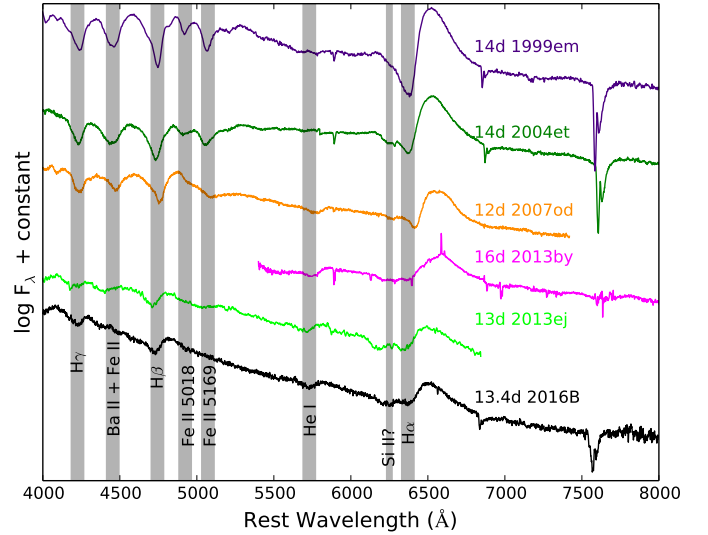
Figure 15. The early spectrum of SN 2016B at 13.4 d is compared with those of type IIP and IIL SNe.
