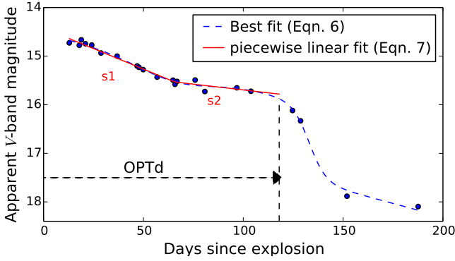
Figure 2. The V-band light curve of SN 2016B fitted with the expression given in Olivares et al. (2010) shown with the (blue) dashed lines. The red lines are from the fit with the piecewise linear function to the light curve with an early declining phase ( s_1 ) and a plateau phase ( s_2 ). The dashed vertical line denotes the end of the plateau phase.
