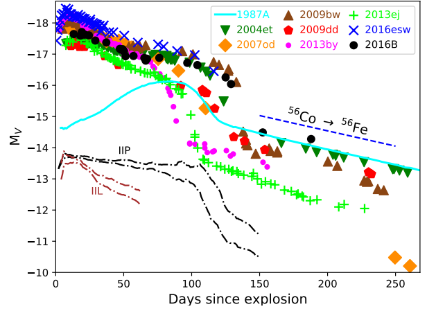
Figure 3. Comparison of absolute V-band light curves of SN 2016B with other Type II SNe. The magnitudes are corrected for distance and reddening as listed in Table 3. The radioactive decay line assuming full trapping of photons is shown with dashed lines. The dash-dotted lines depicts the range of slopes of Type IIP and IIL SNe as presented in Faran et al. (2014).
