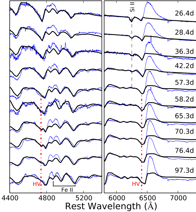
Figure 12. SYN++ modelling of the H Balmer, Fe II and Si II lines in the spectra of SN 2016B shown at the photospheric phases. The broad, extended absorption feature of H I from the 57.3 d spectrum is reproduced using a normal velocity and a high velocity component.
