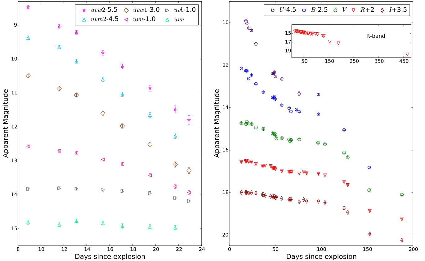
Figure 1. Swift UVOT (left panel) and broadband UBVR (right panel) light curves of SN 2016B shifted arbitrarily for clarity. The inset plot in the right panel shows the R -band light curve up to the last point obtained on 465 d with the 3.6m DOT.
