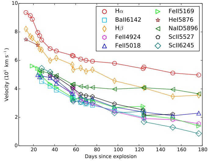
Figure 14. Velocity evolution of the prominent lines in the spectra of SN 2016B estimated from the shift in the P-Cygni absorption feature.
