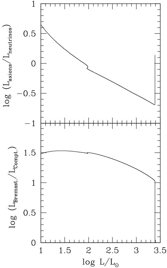
Fig. 2. Upper panel: evolution of ratio between axion and neutrino luminosities, from the base of the RGB ( \log L/L_\odot = 1 ) to the RGB tip, for a model with M = 0.82 M_\odot , Y = 0.25 , and Z = 0.001 . Only the coupling with electrons has been switched on ( g_{13} = 1 ). Lower panel: evolution of the ratio between Bremsstrahlung and Compton axion luminosities.
