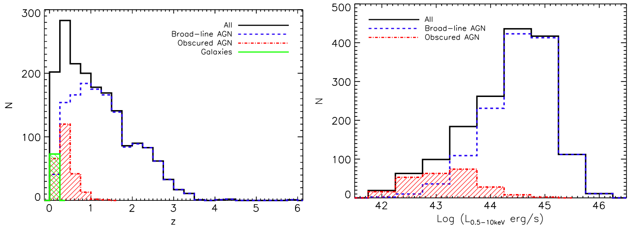
Figure 13. Left: spectroscopic redshift distribution of the 1775 extragalactic Stripe 82X sources, with different classes of objects highlighted. Half the sample is above a redshift of one, and contains predominantly broad-line AGNs at these distances. Nearly all obscured AGNs (i.e., sources optically classified as galaxies with but with full band X-ray luminosities above 10^{42} erg s ^{-1} ) are at a redshift below 1, while the optical and X-ray galaxies are at z < 0.25 (Compton-thick AGNs that have low observed X-ray flux due to heavy obscuration can be included in the “galaxy” bin). Right: observed full-band luminosity distribution for the 1603 spectroscopically confirmed X-ray AGNs (i.e., L_{0.5-10\text{ keV}} > 10^{42} erg s ^{-1} ), where the distribution peaks at high-luminosities ( 44.25 \text{ dex} < \text{Log}(L_{0.5-10\text{ keV}} \text{ erg s}^{-1}) < 45.25 \text{ dex} ). High-luminosity AGNs are predominantly broad-line sources while the lower-luminosity AGNs are mostly obscured. We note that these trends are for the \sim 30\% of the parent Stripe 82X sample that have spectroscopic redshifts and that with increased completeness and more sources identified via photometric redshifts, we expect to confirm more AGNs at all luminosities and redshifts, including at z > 2 and L_{0.5-10\text{ keV}} > 10^{45} erg s ^{-1} , and a higher percentage of obscured AGN.
