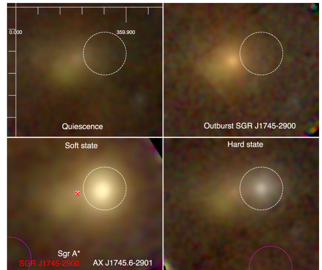
Figure A1. NuSTAR exposure corrected RGB images of AX J1745.6-2901 (red, green and blue show the 3–6, 6–10 and 10–60 keV band, respectively). The white dashed circle shows the region used to extract the spectrum of AX J1745.6-2901. The white and red crosses show the position of Sgr A* and SGR J1745-2900, respectively. The top left-hand panel shows the GC on 2012-07-20, when no bright X-ray transient was observed and AX J1745.6-2901 was in quiescence. The scale is in Galactic coordinates. The top right-hand shows the GC X-ray emission on 2013-04-27, just before the outburst of AX J1745.6-2901 and around the peak of the outburst of SGR J1745-2900. The bottom left-hand and right-hand panels show the X-ray emission on 2015-02-25 and 2014-09-27, while AX J1745.6-2901 was in the soft and hard states, respectively. The magenta dashed circle shows the region used to extract the local background. The same logarithmic colour scale has been applied to all maps.
