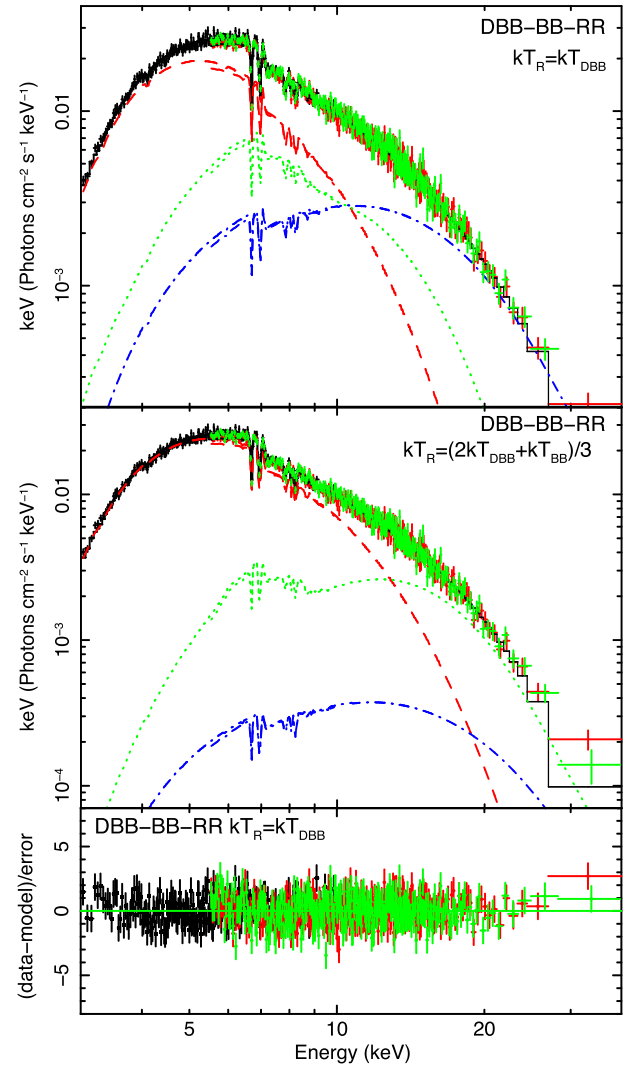
Figure 7. XMM-Newton + NuSTAR spectra of the longest simultaneous soft-state observation, same as Fig. 6. Upper panel: Best-fitting broad-band fit performed with the double thermal plus relativistic ionized reflection model ( DBB-BB-RR ). The dashed red, dash-dotted blue, dotted green and solid black lines show the emission from the disc blackbody, blackbody, relativistically ionized reflection components and total emission, respectively. The reflection spectrum is produced by illuminating the disc with a thermal emission with kT_R = kT_{\text{DBB}} . Middle panel: Same as upper panel, but assuming that the disc is irradiated by a hotter thermal component ( kT_R = (2 \times kT_{\text{DBB}} + kT_{\text{BB}})/3 ). Lower panel: Residual left once the data are fitted with the model shown in the upper panel.
