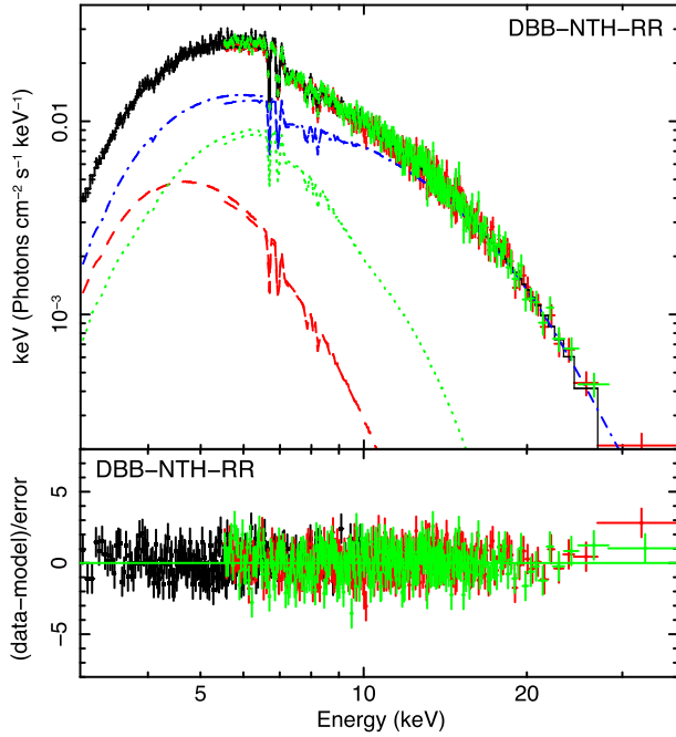
Figure 8. XMM-Newton + NuSTAR spectra of the longest simultaneous soft-state observation (same as Fig. 6), once fitted with the model DBB-NTH-RR. The disc blackbody, Comptonization (NTHCOMP) and ionized reflection (BBREFL) are shown with red dashed, blue dot-dashed and green dotted lines, respectively.
