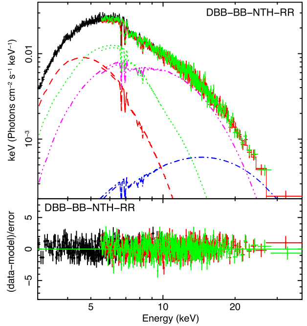
Figure 9. XMM-Newton + NuSTAR spectra of the longest simultaneous soft-state observation (same as Fig. 6), once fitted with the three component model DBB-BB-NTH-RR. The disc blackbody, blackbody, Comptonization (NTHCOMP) and relativistic ionized reflection (BBREFL) are shown with red dashed, magenta dot-dot-dashed, blue dot-dashed and green dotted lines, respectively.
