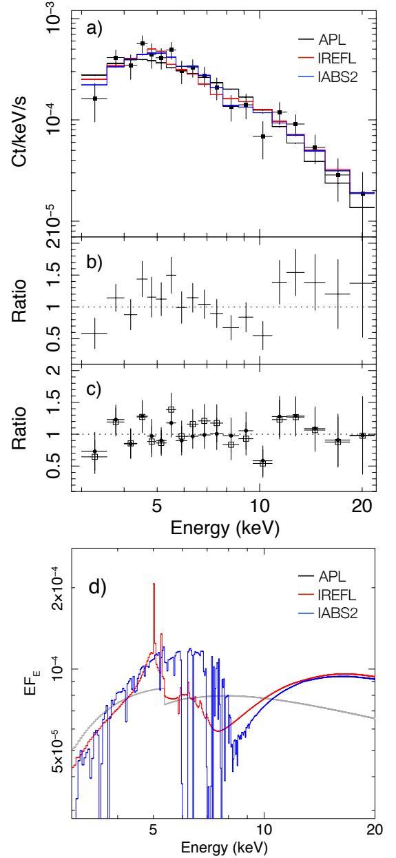
Fig. 5. a) The NuSTAR count rate spectrum of IRAS F00183–7111 in the 3–20 keV band. The three solid-line histograms plotted along the spectral data show best-fit models of the absorbed power-law (black, APL in Table 2) and the reflection spectrum computed by xillver (red, IREFL) and the ionized absorption spectrum (blue, IABS2). All the models are folded through the detector response; b): Data/model ratio for the APL model in a); c) for IREFL (open squares) and IABS2 models (filled circles); and d) The three models shown above, without response folding and plotted in flux units.
