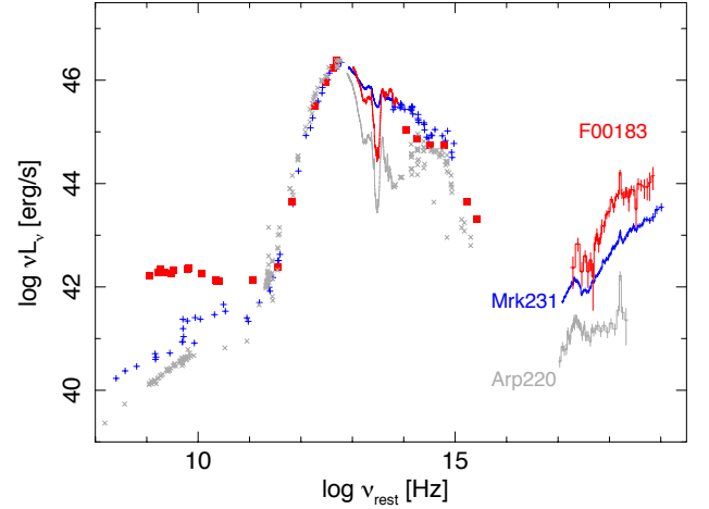
Fig. 7. The radio to hard X-ray spectral energy distribution (SED) of IRAS F00183–7111 (in red). The radio data, sub-millimetre to infrared data, and the optical to UV data are taken from Norris et al (2012, references therein), Spoon et al (2009) and NED, respectively. For comparison, the SEDs of Arp 220 and Mrk 231, normalised to the far-infrared peak of IRAS F00183–7111, are overplotted in light grey and blue, respectively. This gives a convenient way to see the spectral differences between the three SEDs. The Spitzer IRS low-resolution spectra of the three sources are also included. Strong radio and X-ray excess emission from the active nucleus and the mid-IR emission from hot dust are evident in IRAS F00183–7111 and Mrk 231, relative to Arp 220. Note that Mrk 231 is becoming more radio-loud in recent years than those the data plotted (Reynolds 2017).
