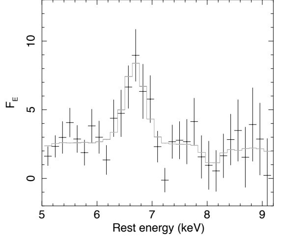
Fig. 2. The rest-frame Fe K band spectrum of IRAS F00183–7111. Data obtained from XMM-Newton EPIC cameras, Chandra ACIS-S, Suzaku XIS, were combined. The data are in flux density in units of 10^{-14} \text{ erg s}^{-1} \text{ cm}^{-2} \text{ keV}^{-1} . The Fe line feature peaks at 6.7 keV and has a moderate width of \sigma \sim 0.15 \text{ keV} . For reference, the blueshifted absorption model for the NuSTAR spectrum discussed in Sect. 3.2.3 (IABS2 in Table 2), supplemented by a Gaussian line for the Fe K feature, is overplotted by the histogram in grey. The continuum level is corrected for the flux difference (see Sect. 3.2.2). The blueshifted Fe xxv absorption line at 8 keV predicted by the absorption model seems to be matched by the data.
