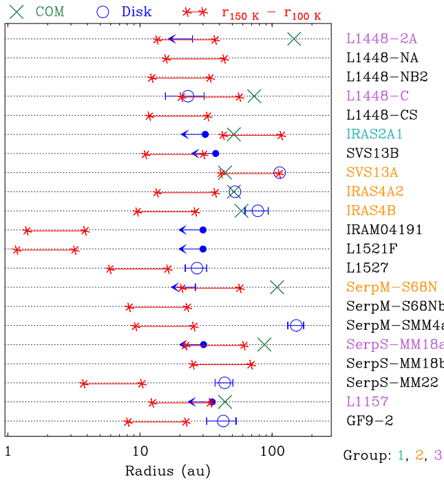
Fig. 13. Comparison of the COM emission radius (green cross) to the disk radius (blue circle, with error bar when available) and the range of radii over which ices are expected to sublimate from the grain mantles (red bar terminated by stars). The COM emission radius corresponds to half the FWHM size reported in Table 4, when COMs are detected. The disk radius corresponds to half the FWHM size derived by Maury et al. (2019) when they detect a candidate disk-like structure, corrected for the new distance when needed. The radii of the candidate disk-like structures for SVS13A (circumbinary in this case) and IRAS4A2 come from a similar analysis (A. Maury, priv. comm.). A blue dot with an arrow pointing to the left indicates the upper limit on the radius of a detected but unresolved disk. A blue bar with an arrow pointing to the left represents a disk nondetection with an upper limit on the radius that could still be estimated by Maury et al. (2019). All disk parameters were rescaled to the new distances when necessary. For each source, the two red stars mark the temperature range 100–150 K (from right to left) expected from the luminosity given in Table 1. The names of the sources belonging to groups 1, 2, and 3 are color-coded with the color scheme indicated in the bottom right corner, as in the case of the frames in Fig. 6 and as described in Sect. 3.7.
