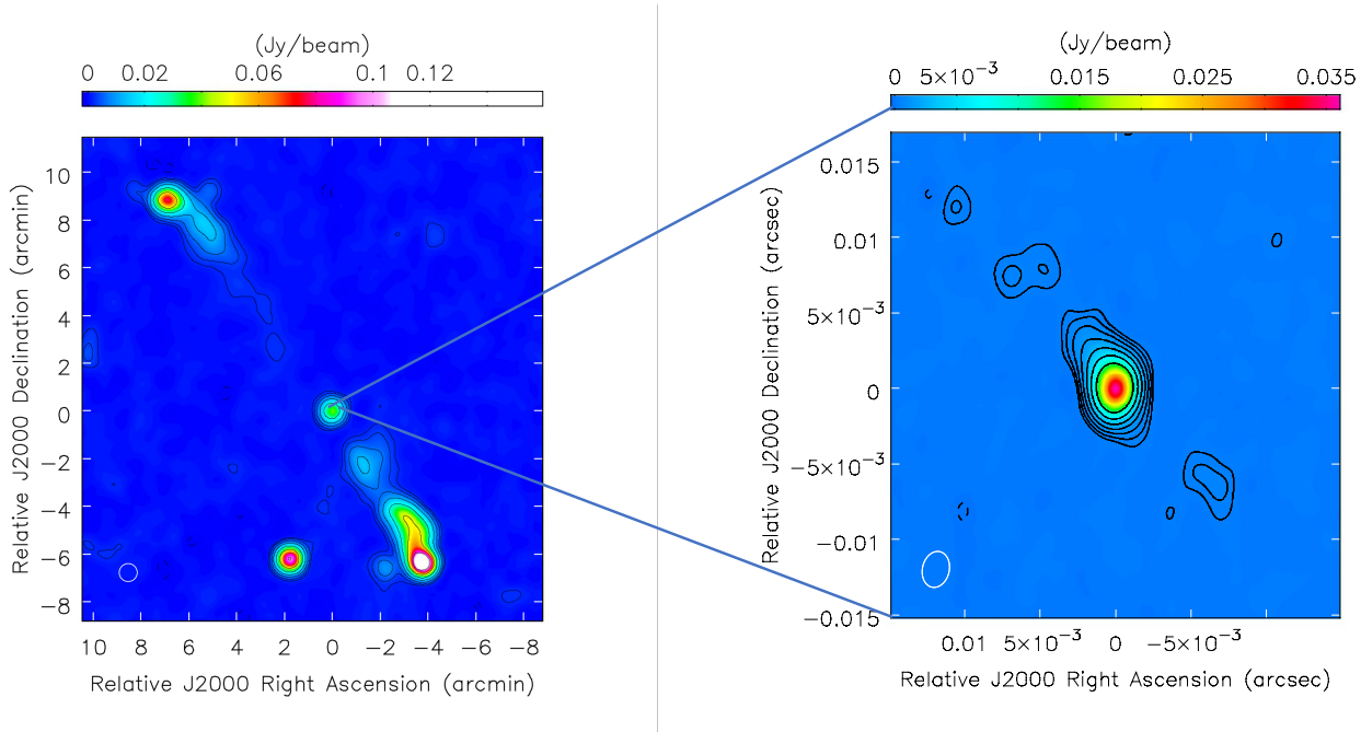
Figure 1. (Left) NVSS image of Mrk1498, at 1.4 GHz. Contours are 3\sigma multiples (-1, 1, 2, 4, 8, 16, 32, 64). The RMS is 0.5 mJy/beam, while the beam ( 45 \times 45 arcsec) is plotted in the lower-left corner, and (right) zooming image of the nucleus with VLBA at 4.8 GHz from archival data. Contours are 3\sigma multiples (-1, 1, 2, 4, 8, 16, 32, 64). The RMS is 0.06 mJy/beam, while the beam ( 2.41 \times 1.78 mas) is plotted in the lower-left corner. Not at scale.
