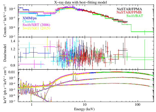
Figure 10. Upper panel: X-ray spectrum from XMM/pn (blue), Chandra (cyan), 2006 Swift /XRT (magenta), 2015 Swift /XRT (yellow), NuSTAR/FPMA (black), NuSTAR/FPMB (red) and Swift /BAT (green), plotted with the best-fitting model. Middle panel: Data/model ratio. Lower panel: Best-fitting Borus model including the unabsorbed power law and MEKAL. The data were binned for plotting purposes.
