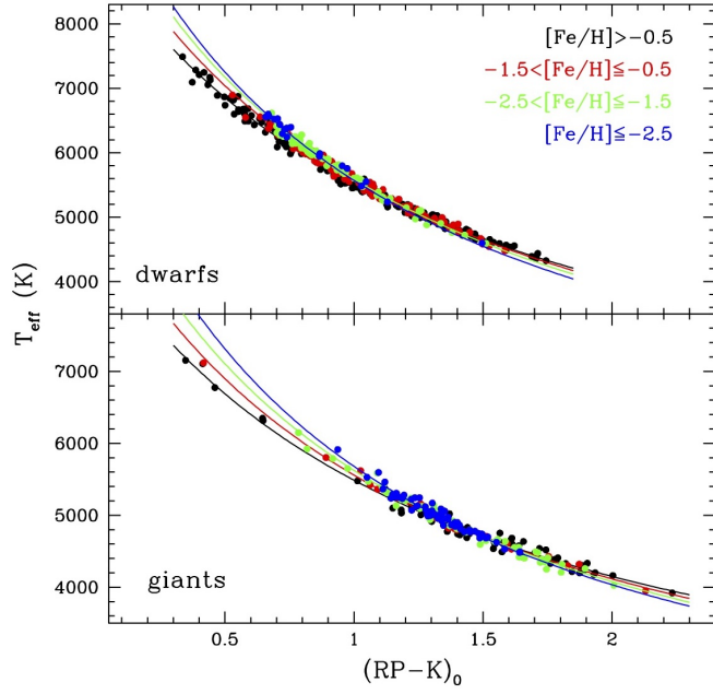
Fig. A.6. Same as Fig. A.1 but for the (RP - K_s)_0 colour.
