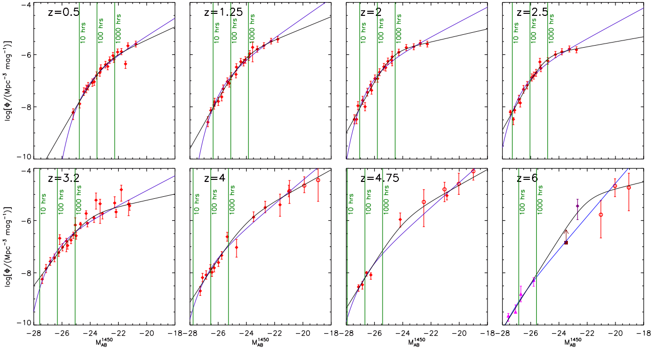
Figure 1. Evolution of the UV LF \log \Phi (\text{Mpc}^{-3} \text{ mag}^{-1}) as a function of the absolute magnitude M_{\text{AB}}^{1450} , from z = 0.5 to 6. In each panel, symbols represent observational data with the corresponding error bars (Jiang et al. 2009: magenta triangles; Fiore et al. 2012: purple diamond; Giallongo et al. 2012 and references therein. 2015: red circles, filled and open, respectively; Kashikawa et al. 2015: dark red square), while the solid curves represent our best-fitting parametrization of the QSO LF using a DPL function (black) and a Schechter function (blue). In each panel, the green vertical lines indicate the 5\sigma detection thresholds with SKA-MID at \nu = 13.8 GHz, in 10, 100 and 1000 h of observing time.
