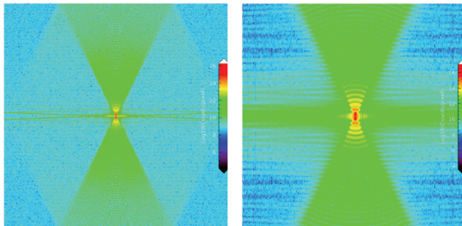
Figure 11: the focus of a perfectly aligned Wolter collimator. Left: in X-rays at 1.2 keV ( \lambda = 1 nm), 0.5 mm wide detector. Right: in UV light, ( \lambda = 0.2 \mu m), 5 mm wide detector. Log color scale.
