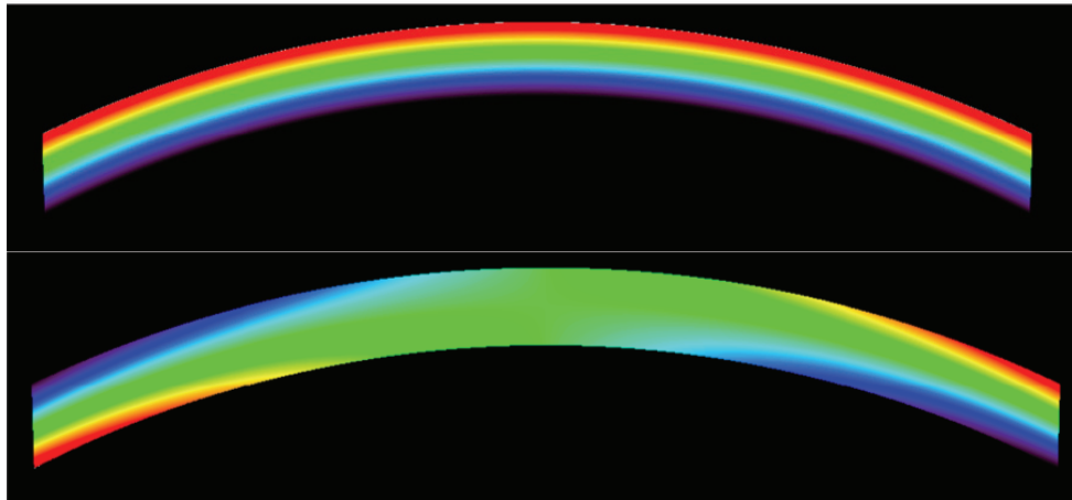
Figure 10. OPD maps (the \varepsilon(\mathbf{r}_1) term in Eq. 8) in linear color scale, as resulting from two possible misalignments of the parabola with respect to the hyperbola. Top: misalignment in pitch. Bottom: Misalignment in yaw (see Figure 12 for the reference frame).
