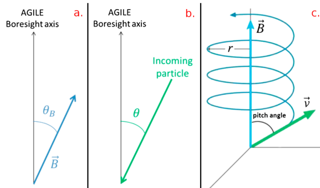
Figure 7. Definition of angles in the AGILE-GRID frame. (a) \theta_B : the angle between the local magnetic field and the AGILE boresight axis. (b) \theta : the angle between the incoming particle track and the AGILE boresight axis (top incoming on-axis particles have \theta = 0 ). (c) Pitch angle: angle between the particle track and the local geomagnetic field.
