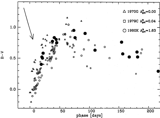
Fig. 4. Comparison of the B-V color curve of SN 1990K with those of well studied Linear SNI. The latter have been corrected only for galactic extinction. The arrow indicates the shift applied to the observed data of SN 1990K to best fit the average color curve of SNIIL. We conclude that SN 1990K suffered a color excess E(B-V)=0.5 \pm 0.1 mag and, most likely, was discovered about 15 days after maximum
