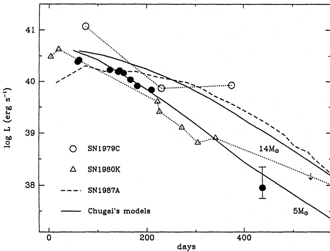
Fig. 11. Evolution of the luminosity of H\alpha for SN 1990K (filled circle) compared with the same data for SN 1979C, SN 1980K and SN 1987A. Also reported are the Chugai's 5 and 14 M_{\odot} models (Chugai 1991)
