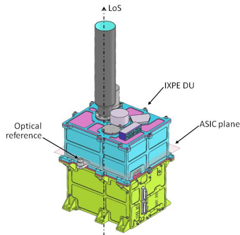
Figure 1 IXPE Detector Unit (DU) assembly with one of the three coplanar optical reference shown.
