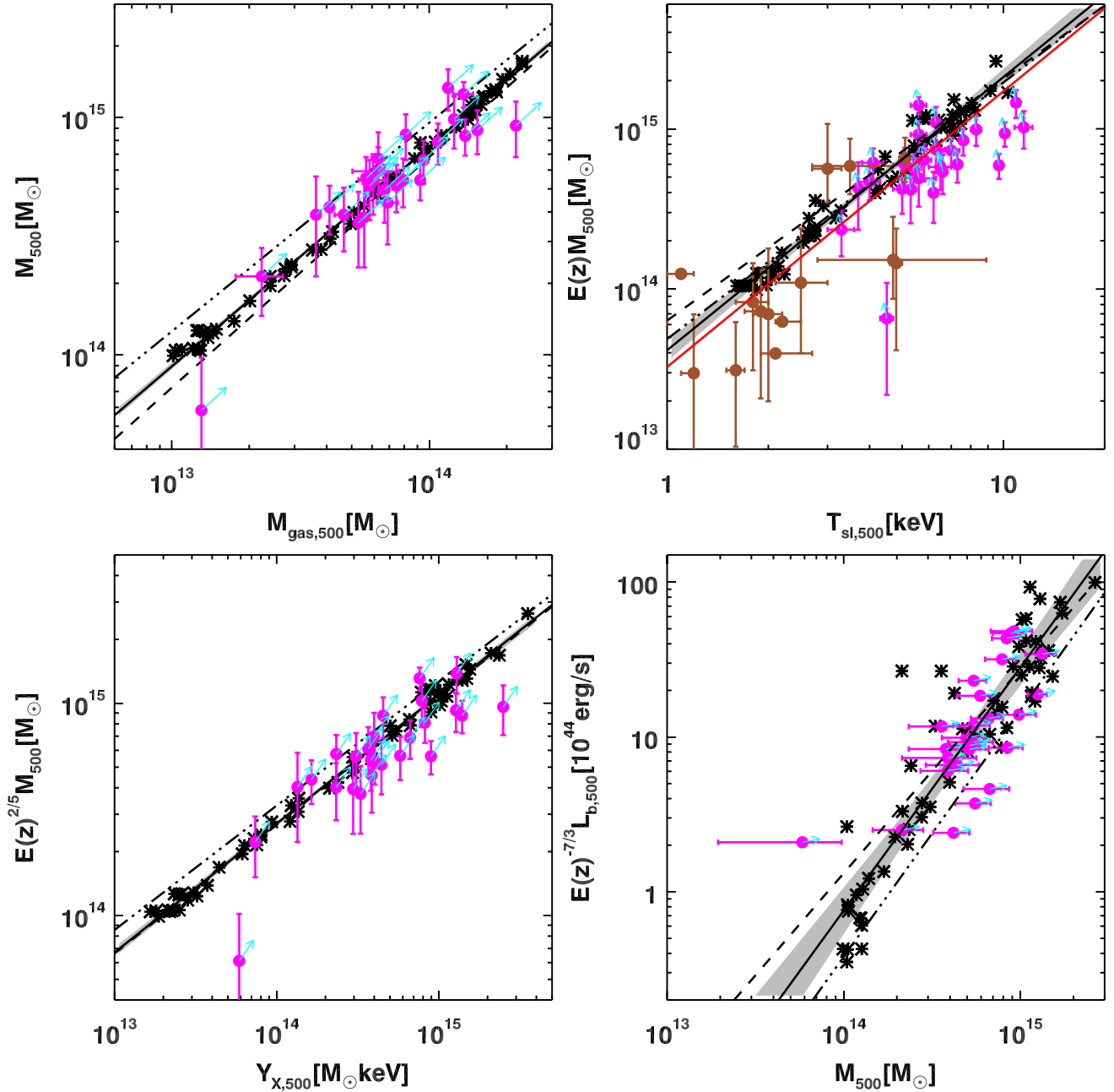
Figure 2. Comparison between scaling relations at z = 0 and those derived from local observations ( z < 0.25 ). In clockwise order, we plot the M-M_g , M-T_{sl} , L-M and M-Y_X relations. The observational data are taken from Mahdavi et al. (2013) and Mahdavi et al. (2014, , magenta), and Lieu et al. (2016, , brown). They are shown with 1\sigma error bar. The cyan arrows associated with the Mahdavi et al. points represent the change of the quantities after correcting (i) the total mass by 25 per cent as suggested by Hoekstra et al. (2015) and (ii) the other quantities by the amount estimated within our AGN sample (see the text for details). In each panel, the solid black line represents the best-fitting relation of the AGN sample shown with black asterisks; the grey shaded area is the associated 1\sigma scatter around the best fit; the dashed and dash-dotted lines represent the best-fitting relations of the NR and CSF runs, respectively. The luminosities are bolometric, none of the simulated and observed quantities is core-excised, and the observed data are rescaled to the cosmology adopted in the simulation.
