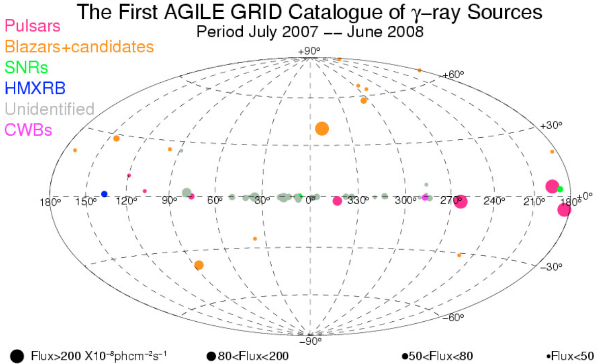
Fig. 3. The First AGILE-GRID Catalog of high-confidence sources, plotted in in Aitoff projection and galactic sky coordinates. Symbol sizes are proportional to source flux values, and symbol colors indicate different source classes.
