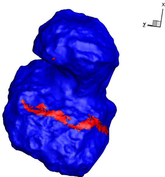
Figure 7. Inferred trajectory footprint location of those particles that could contribute to the jet brightness shown in Fig. 3. The footprints, marked in red, are concentrated in an area outside of the maximum water source rate region shown in Fig. 1. The inferred trajectory footprint location area is consistent with that of the active pits in the Seth region, as determined by Vincent et al. (2015).
