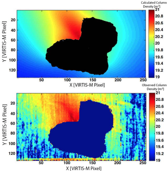
Figure 2. Comparison of the \text{H}_2\text{O} column density ( \text{m}^{-2} ) map observed by Rosetta VIRTIS-M [observation I1_00387442903, Migliorini et al. (2016)] with that from our previous kinetic modelling of the coma by Fougere et al. (2016). The surface distribution of the water vapour flux used in the analysis presented in this paper, and this figure are adapted from Fougere et al. (2016). Modelled column density is shown in the top panel and the observed one is shown in the bottom panel. X- and Y-axes represent the instrument pixel grid.
