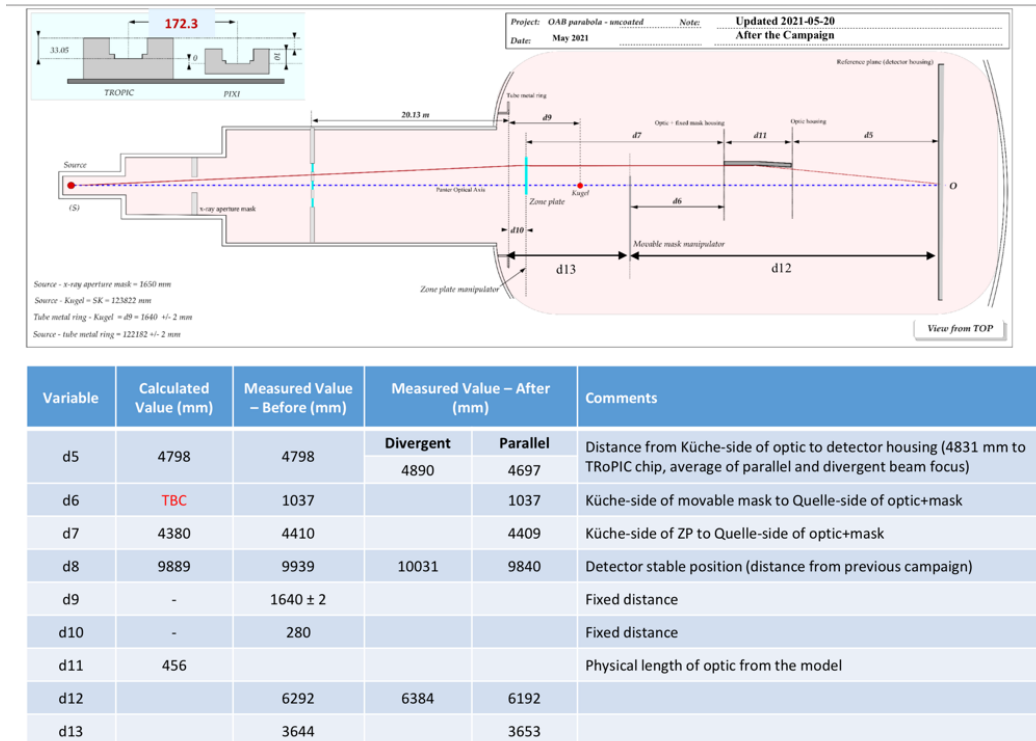
Figure 17: distances measured after venting the chamber, with the detector and the mirror still aligned in the best focus position with the parallel beam.
