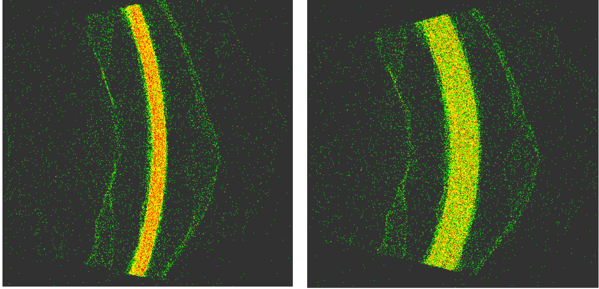
Figure 24: the coated mirror, out-of-focus under diverging X-rays at 1.49 keV. Left: intrafocal image by 384 mm, pitch = + 12.4 arcmin. Right: extrafocal image by 150 mm, pitch = 15.1 arcmin.
