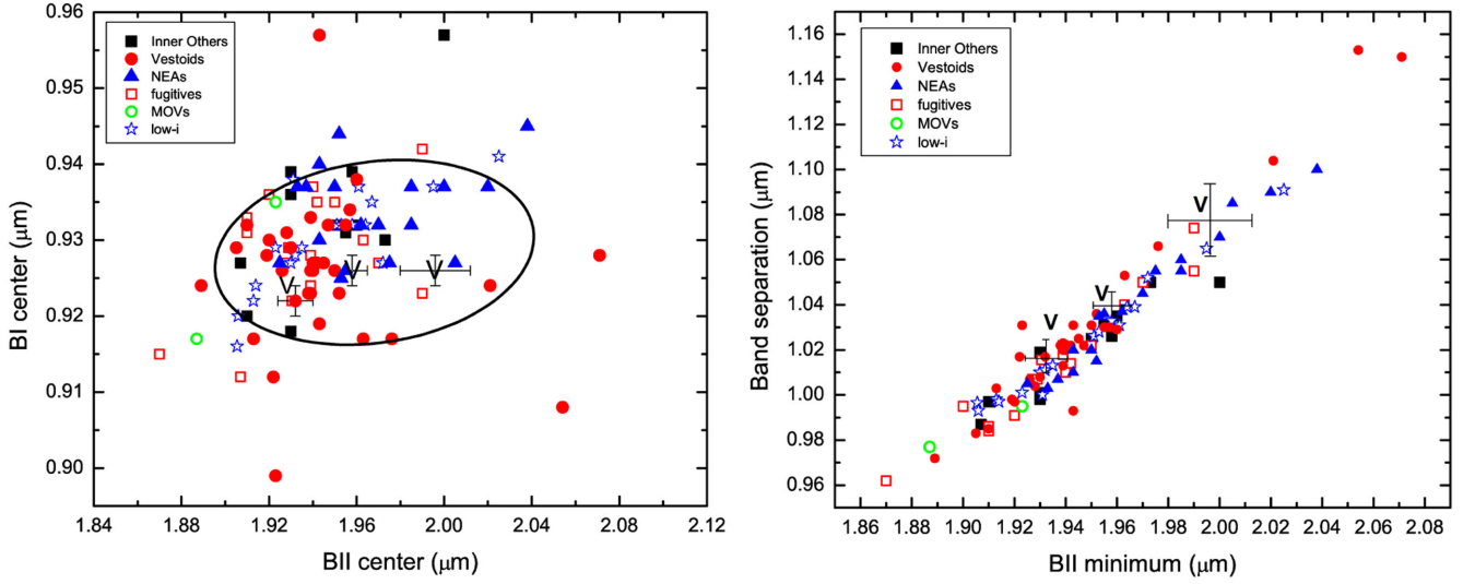
Figure 2. Left-hand panel: BI centre versus BII centre for the different dynamical classes and subclasses of V-types considered in this work: IOs, Vestoids, NEAs, fugitives, MOVs, and low-i (see the main text for details). The V symbols indicate Vesta ground-based observations from Vernazza et al. (2005) while the oval area delimits the range of values obtained by the Dawn spacecraft (De Sanctis et al. 2012). Right-hand panel: Band separation versus BII minimum for the same V-type classes and subclasses considered in the left-hand panel.
