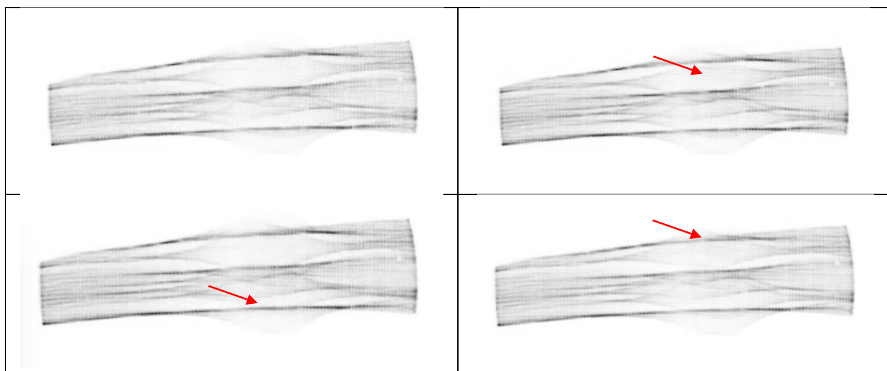
Fig. 15: first sector of the XSM: illuminated at 0.3 keV: activation in sequence of the 7 piezos at -60 V, at 1.4 deg incidence angle. We show (arrows) the activation of the 7 th (top right), the 2 nd (bottom left), and the 8 th (bottom right). The local deformations introduced by the piezos is reduced as they are energized at negative voltages.
