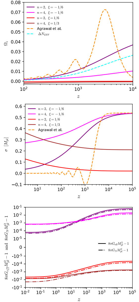
FIG. 1. We plot the evolution of the energy injection \Omega_i := \rho_i/\rho_c (top), the scalar field (center), and the deviation from one of the effective (solid lines) and cosmological (dot-dashed lines) Newton constants (bottom) for the models with n = 2 , \xi < 0 (purple lines), n = 4 , \xi < 0 (magenta lines), n = 2 , \xi > 0 (red lines), and n = 4 , \xi > 0 (brown lines), together with the EDE model of Ref. [27] (orange lines) and the \Lambda CDM + N_{\text{eff}} model (cyan lines). In order to compare the evolution of our model to the aforementioned ones, we set the cosmological parameters to the best fit values in Table 3 of Ref. [27] and set \xi = -1/6 . In the cases with \xi > 0 , we change the values of the initial conditions on the scalar field and the coupling \xi as in the plot legends.
