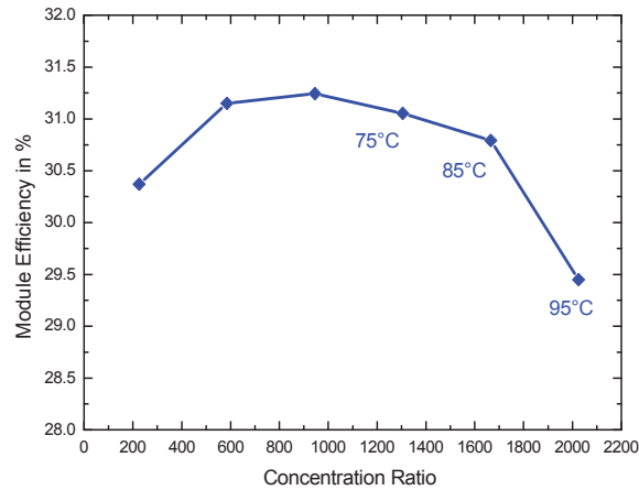
FIGURE 3. Concentration-Ratio dependence of \eta_{\text{mod}} delivered from the our prototype HCPV module. The indoor irradiance measured from the pyrheliometer varied from 580 W/m 2 to 620 W/m 2 during the tests. The temperatures indicated are that measured with the PT100 sensor.
