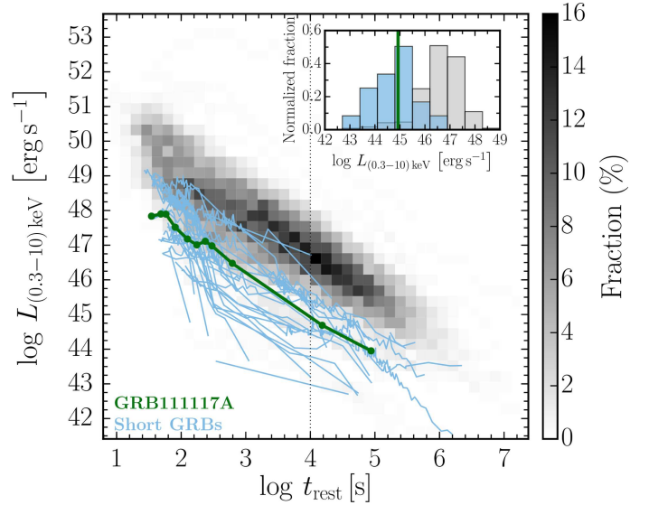
Fig. 5. Rest-frame XRT light curve of GRB 111117A, compared to the general population of GRBs. The gray shaded region is a compilation of long GRB light curves (Evans et al. 2007, 2009), where the color represents density. The light blue lines are sGRB light curves from bursts with duration of T_{90} \lesssim 2 s and those that were classified as short in Kann et al. (2011), Berger (2014) and D’Avanzo et al. (2014). The thick green line is GRB 111117A. Despite the remarkably high redshift, the luminosity is comparable to the bulk of the short burst population, and subluminal compared to the IGRB population. The inset shows the X-ray luminosity distributions of sGRBs and IGRBs at 10 ks, indicated by the vertical dashed line in the main panel.
